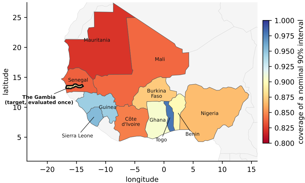
Out-of-country coverage, by held-out country
