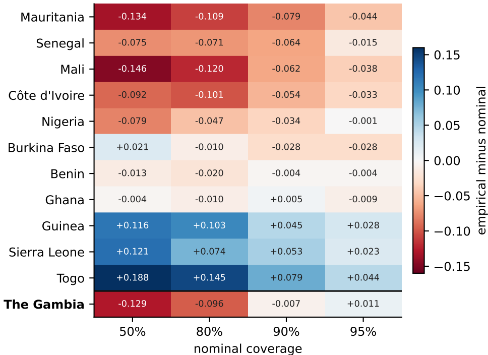
Coverage minus nominal, split conformal
