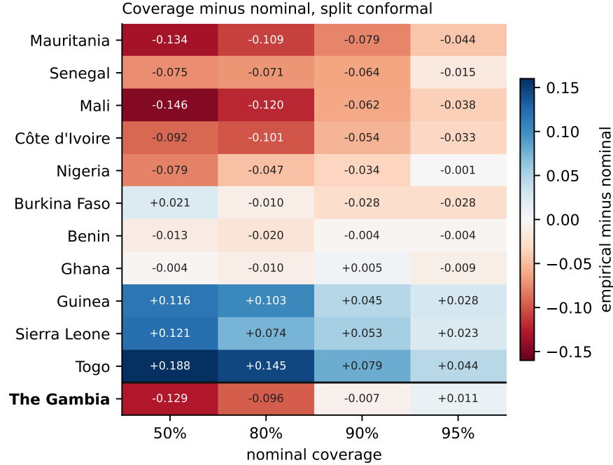
Figure 5: Empirical minus nominal coverage, split conformal, by country and nominal level. Both post-hoc observations are visible at once. Reading down a column gives the dispersion across countries, from Mali at -0.146 to Togo at +0.188 at nominal 50%. Reading along a row gives the level dependence: for almost every country the deviation shrinks as the nominal level rises. The Gambia, below the rule, shows that pattern clearly, at -0.129 , -0.096 , -0.007 and +0.011 .
