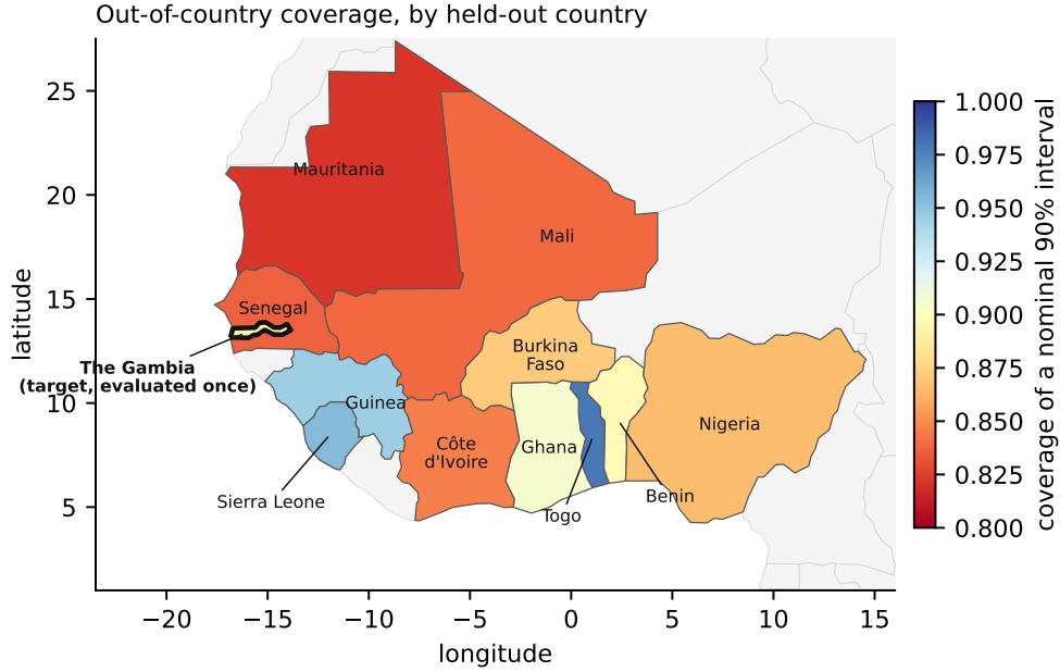
Figure 4: The twelve surveys, shaded by out-of-country coverage of a nominal 90% interval. The Gambia is outlined and was evaluated once. The failures are not uniformly distributed: the Sahelian countries at the top of the map undercover and the wetter coastal countries overcover. That apparent gradient was noticed by inspecting this figure and is treated as a lead in Section 6, not as a result.
