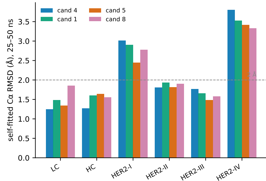
(a) Per-domain RMSD — all folded
