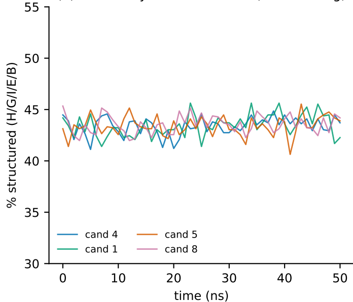
(b) Secondary structure — flat (no unfolding)
