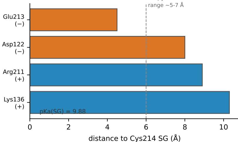
(a) Static site — acidic, no proximal base
