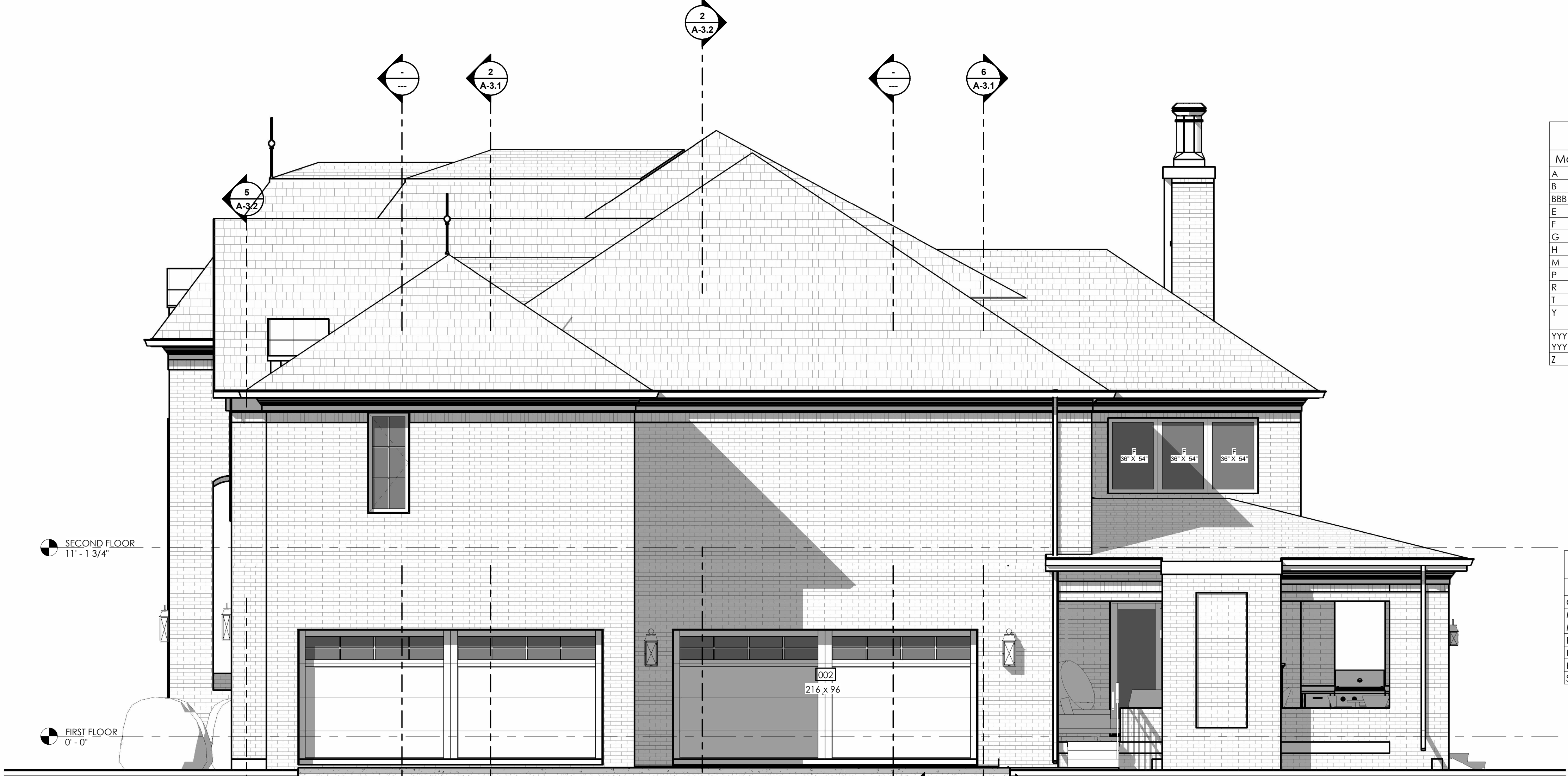
3 NORTH ELEVATION A-2.1 SCALE: 1/4" = 1'-0"
