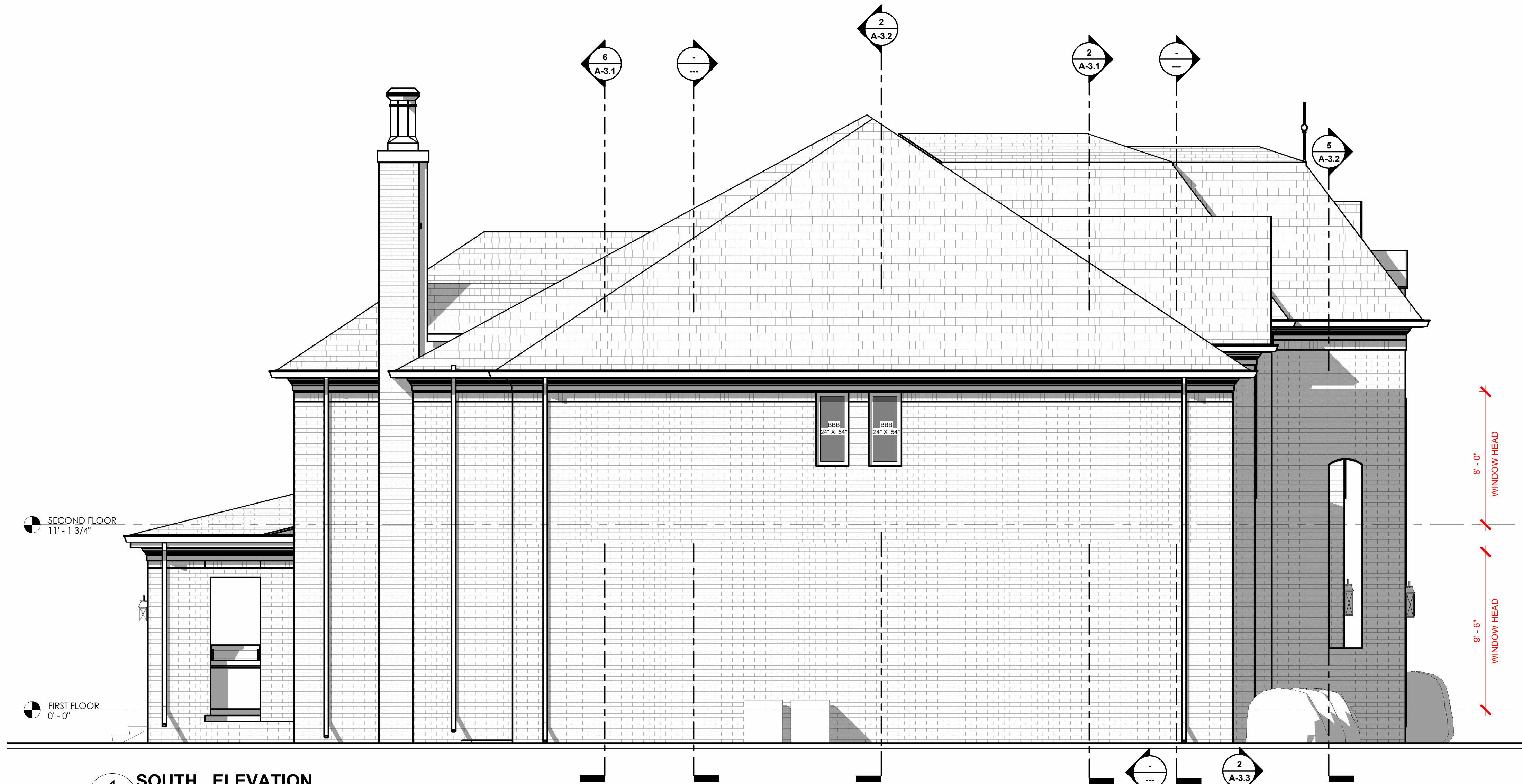
1 SOUTH ELEVATION A-2.2 SCALE: 1/4" = 1'-0"
