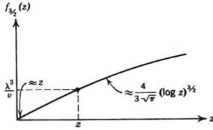
Figure 1: f_{3/2}(Z)
