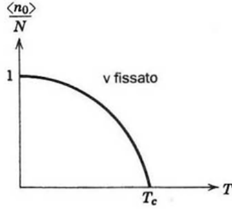
Figure 3: \mathcal{N}_0/\mathcal{N} vs T per T < T_c
