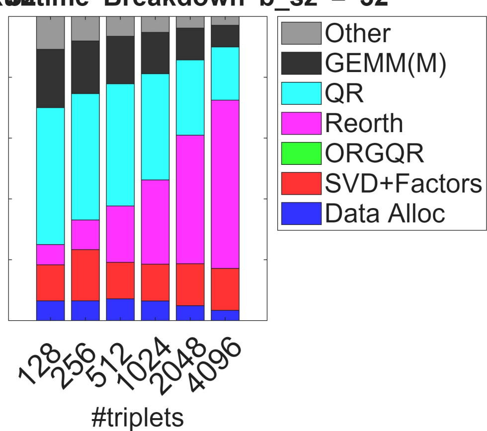
ABRIK - R32 Runtime Breakdown b_sz = 32
