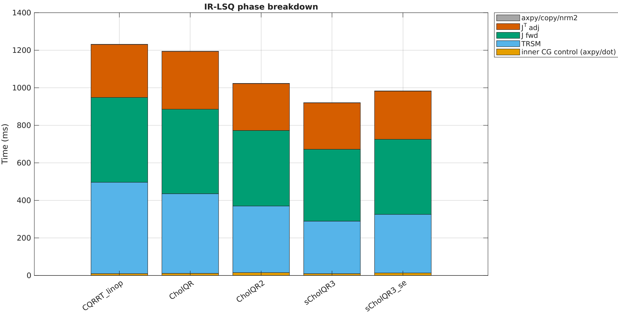
IR-LSQ runtime breakdown — Sparse IR-LSQ Benchmark — 75824 \times 8304 — \kappa \approx 8.8e5 [sd]
