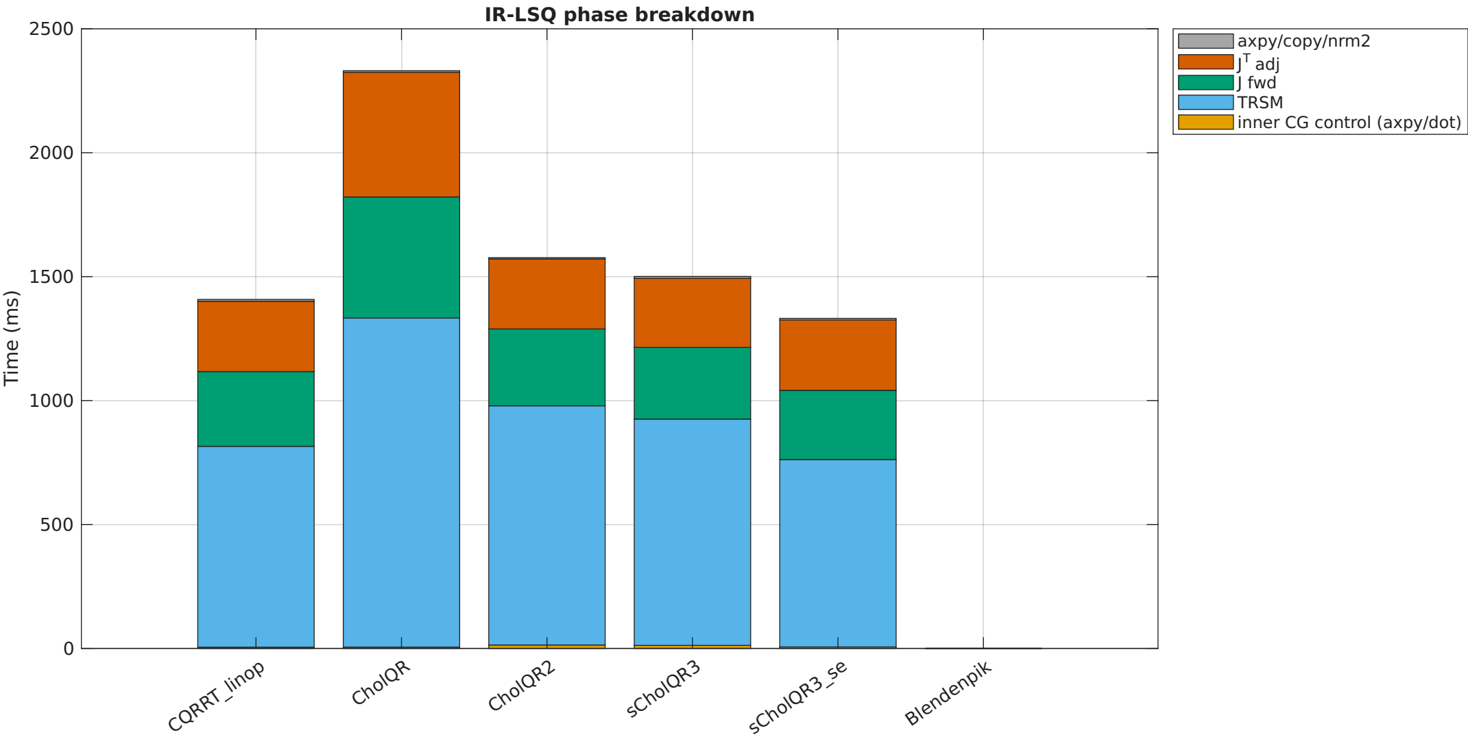
IR-LSQ runtime breakdown — Sparse IR-LSQ Benchmark — 301864 \times 33024 — \kappa \approx \kappa^{\text{colnorm}} \approx 1e6 [dd]
