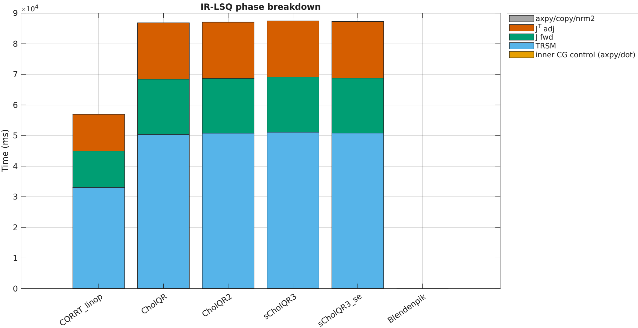
IR-LSQ runtime breakdown — Sparse IR-LSQ Benchmark — 301864 \times 33024 — \kappa \approx \kappa^{\text{colnorm}} \approx 1\text{e}6 [sd]
