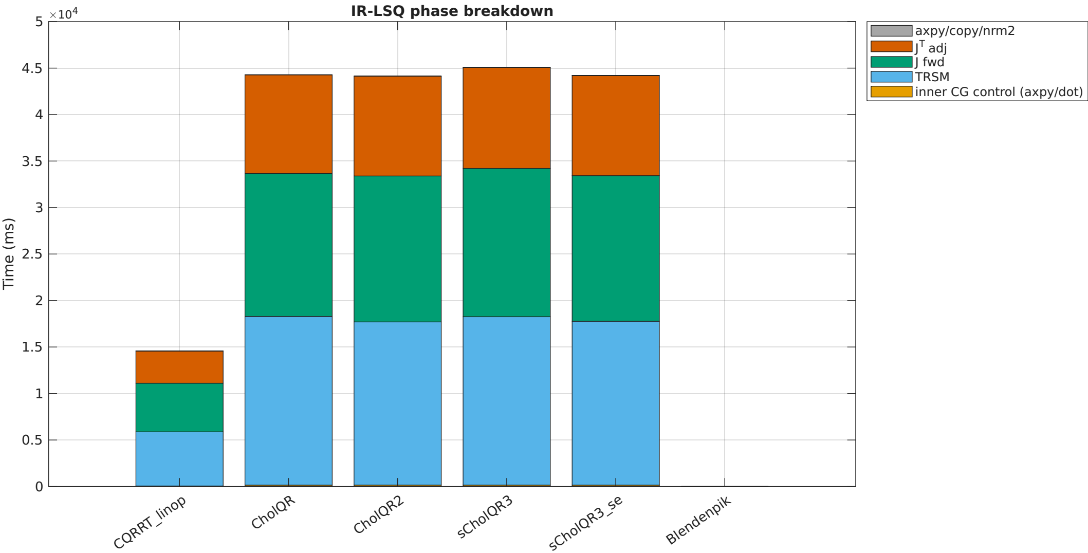
IR-LSQ runtime breakdown — Sparse IR-LSQ Benchmark — 75466 \times 8256 — \kappa \approx \kappa^{\text{colnorm}} \approx 1\text{e}6 [sd]
