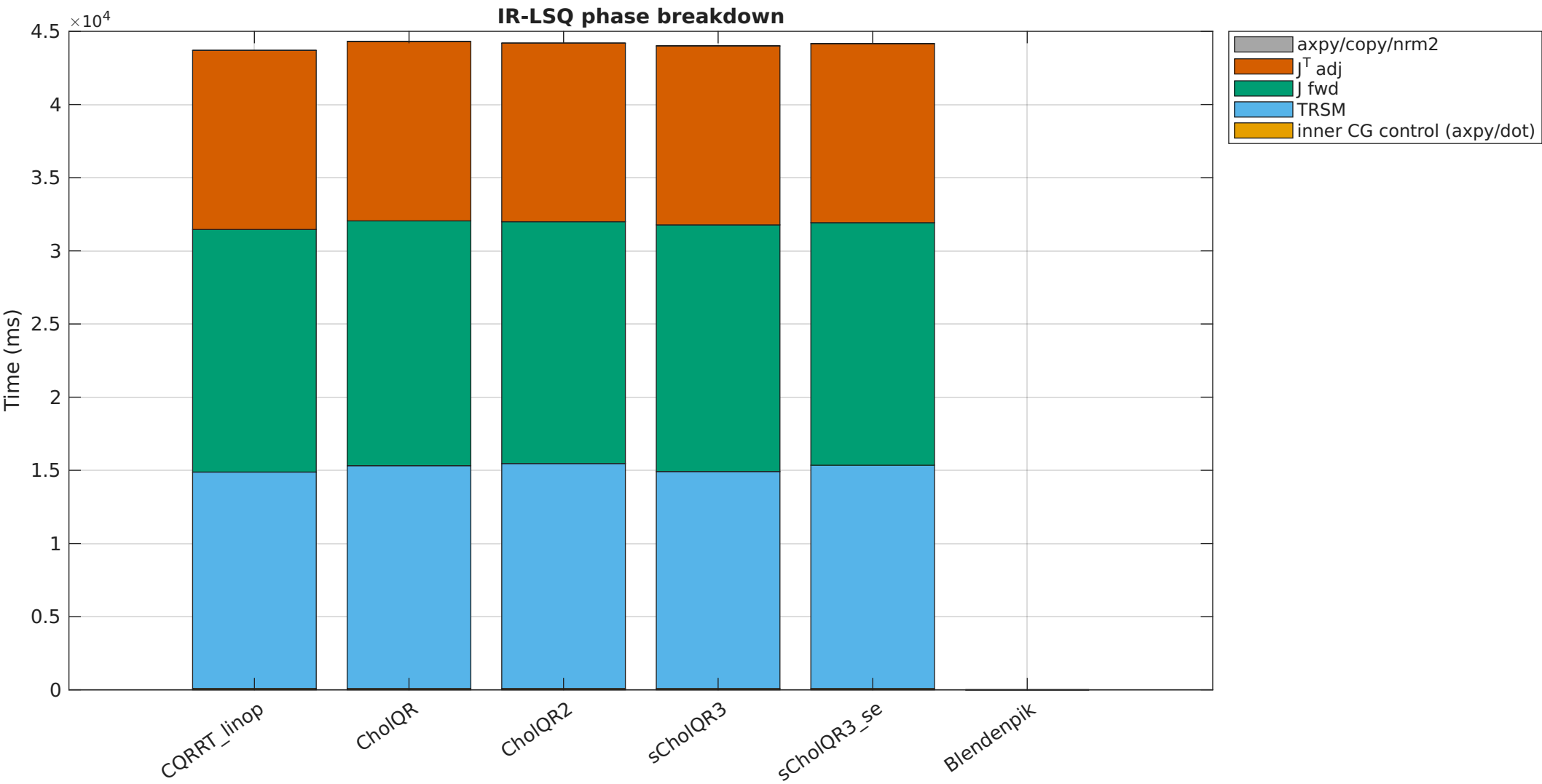
IR-LSQ runtime breakdown — Sparse IR-LSQ Benchmark — 75466 \times 8256 — \kappa \approx \kappa_{\text{colnorm}} \approx 1\text{e}6 [ss]
