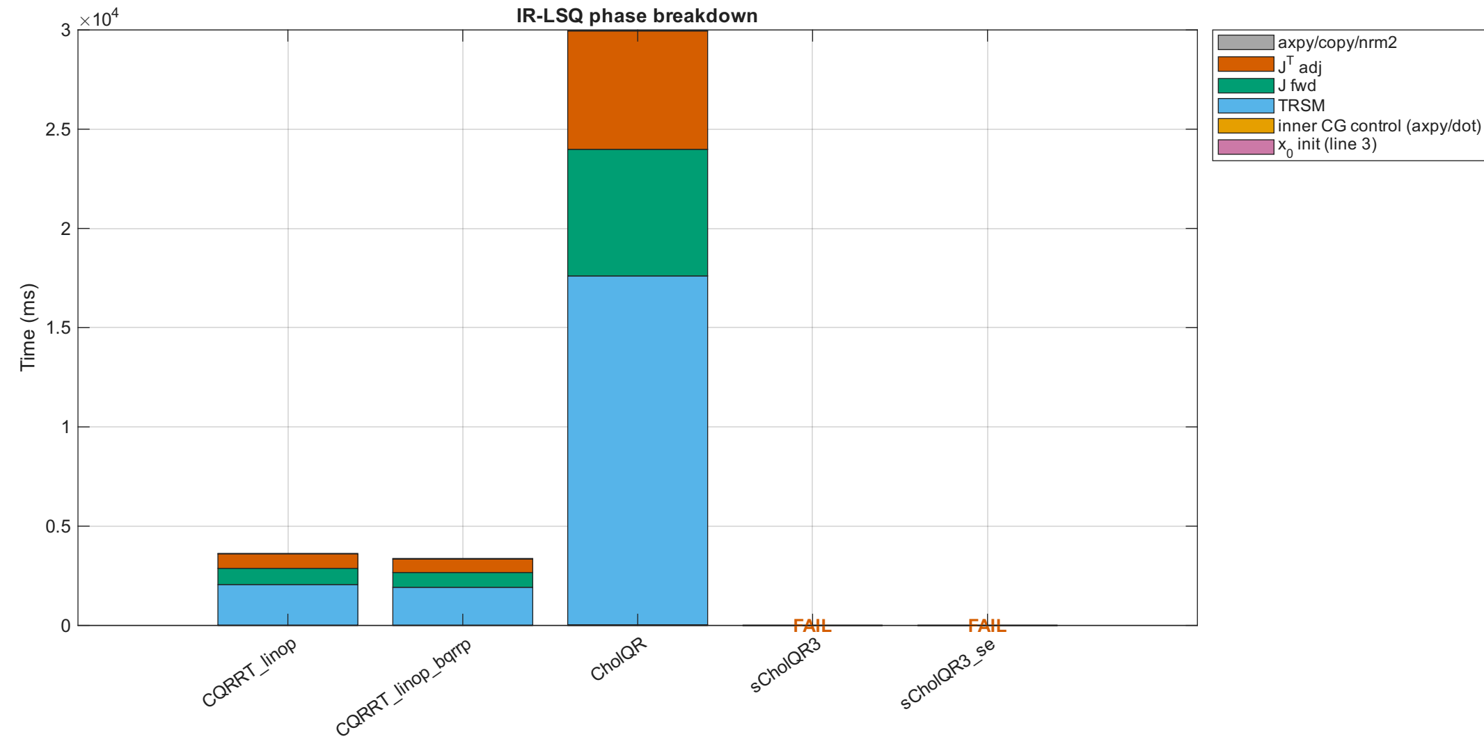
IR-LSQ runtime breakdown — Sparse IR-LSQ Benchmark — 303296 \times 33216 — FEM problem 2 large (303296x33216)
