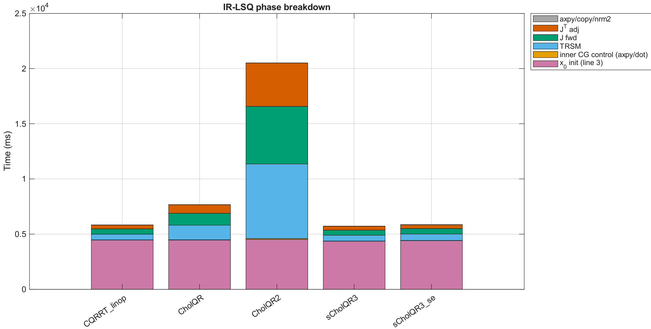
IR-LSQ runtime breakdown — Sparse IR-LSQ Benchmark — 75824 \times 8304 — FEM p roblem 2 small (75824x8304)
