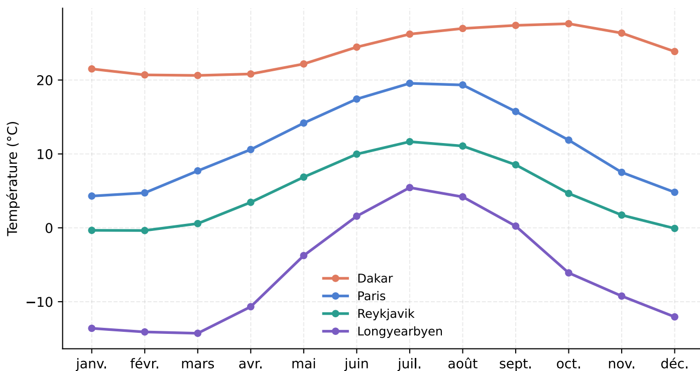
Normale mensuelle 1991-2020 — Dakar, Paris, Reykjavik, Longyearbyen
