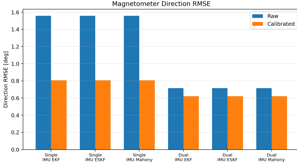
Figure 7: Magnetometer direction RMSE before and after calibration with ESKF included.
