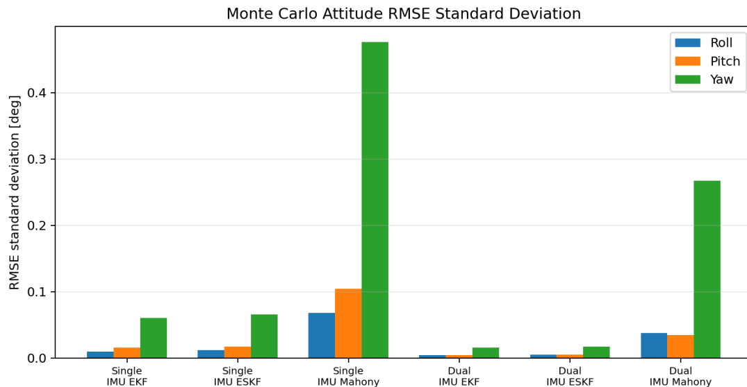
Figure 3: Monte Carlo standard deviation of attitude RMSE with ESKF included.
