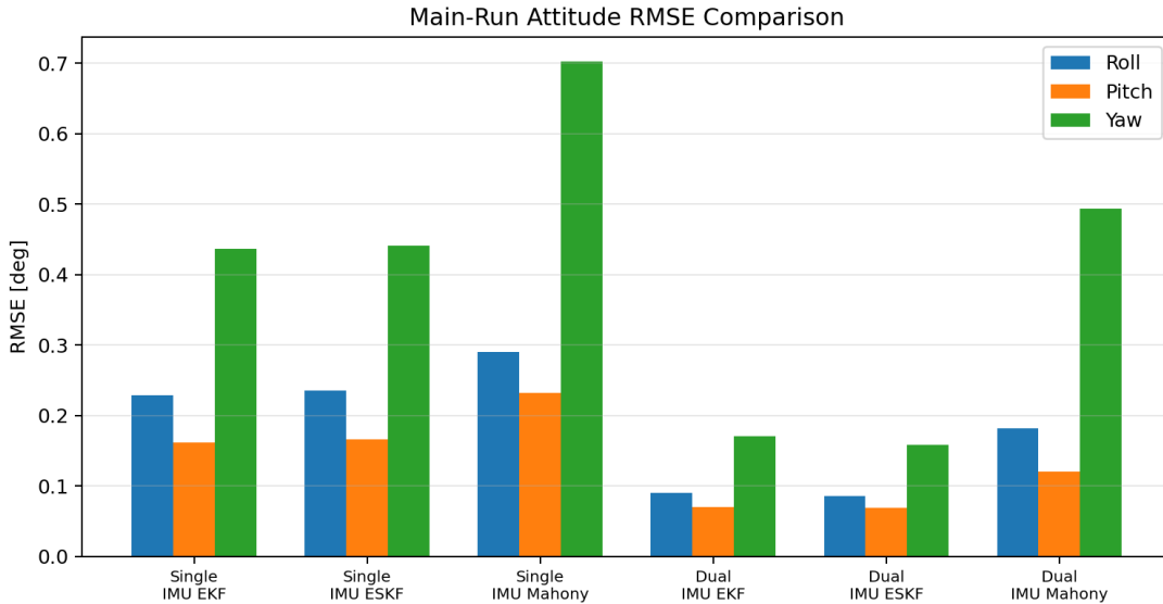
Figure 1: Main-run attitude RMSE comparison with EKF, ESKF, and Mahony included.
