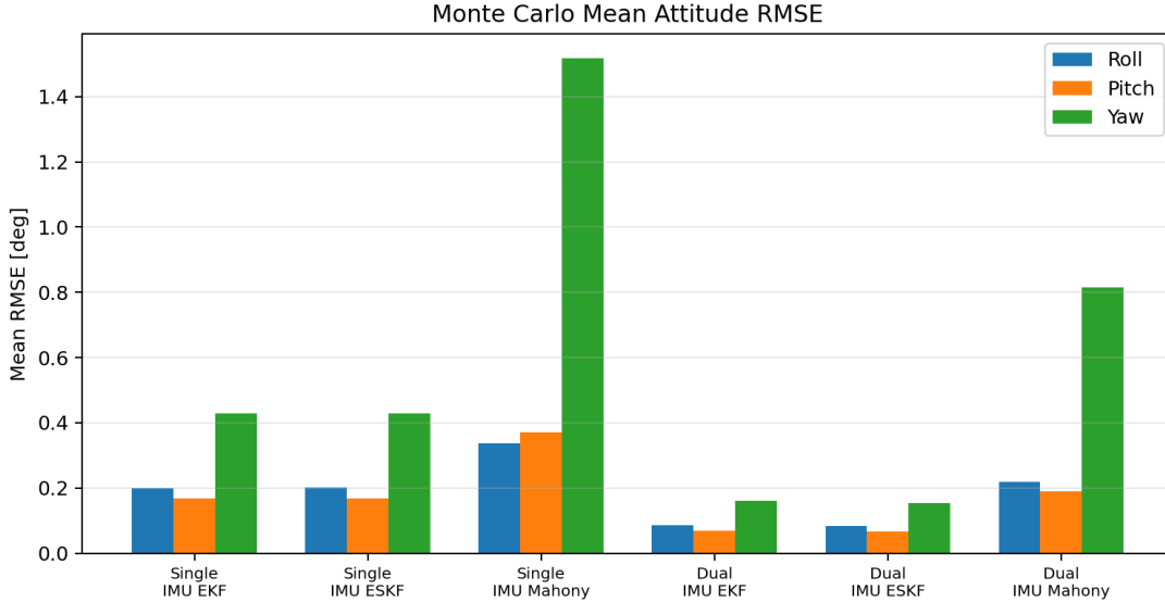
Figure 2: Monte Carlo mean attitude RMSE with EKF, ESKF, and Mahony included.
