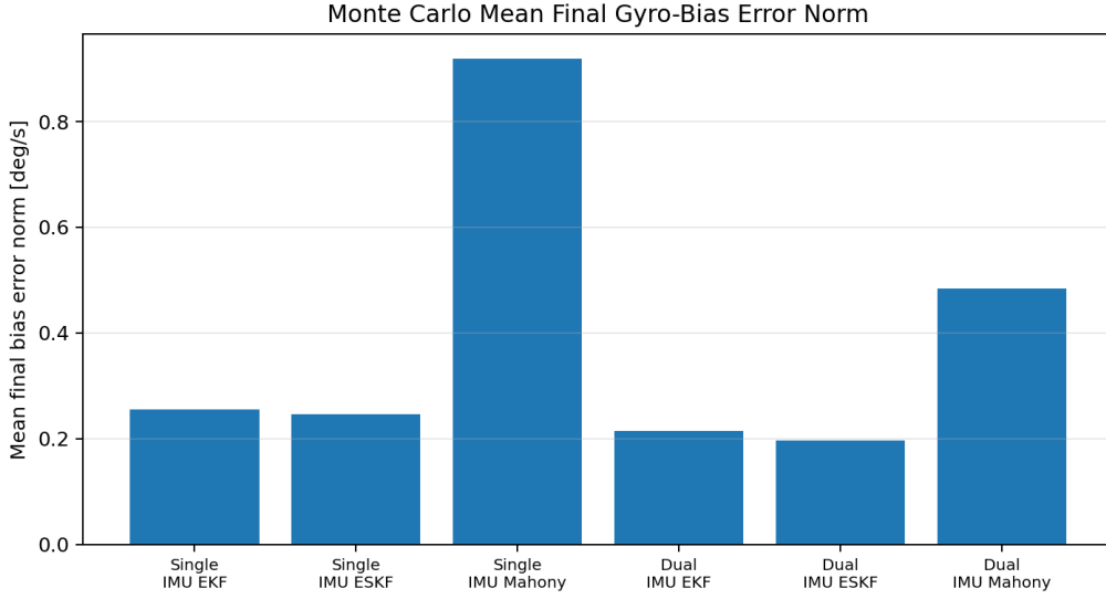
Figure 6: Monte Carlo mean final gyro-bias error norm with ESKF included.
