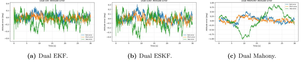
Figure 5: Time-domain attitude error for the three dual-IMU filters.
