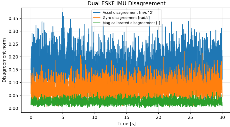
Figure 8: Dual-IMU disagreement metrics for the Dual ESKF main run.
