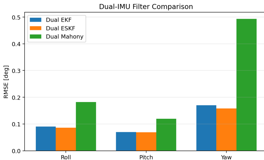
Figure 4: Dual-IMU EKF, ESKF, and Mahony attitude RMSE in the main run.
