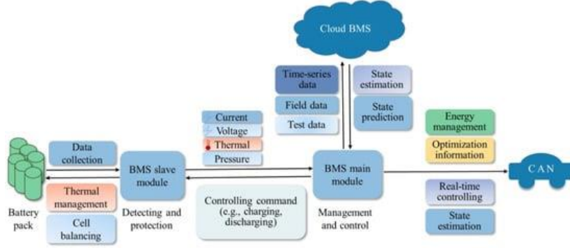
Figure 6 Cyber system: Cloud-based battery modeling (Shi et al., 2023)
