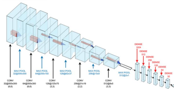
Figure 8 The general architecture of CNN (Ciccarelli et al., 2023)
