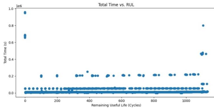
Figure 20 The real data in terms of Total time vs RUL.
