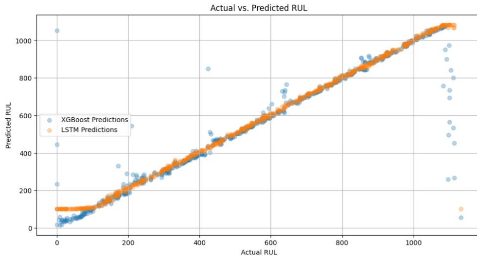
Figure 30 Comparison of XGBoost predictions and LSTM predictions
