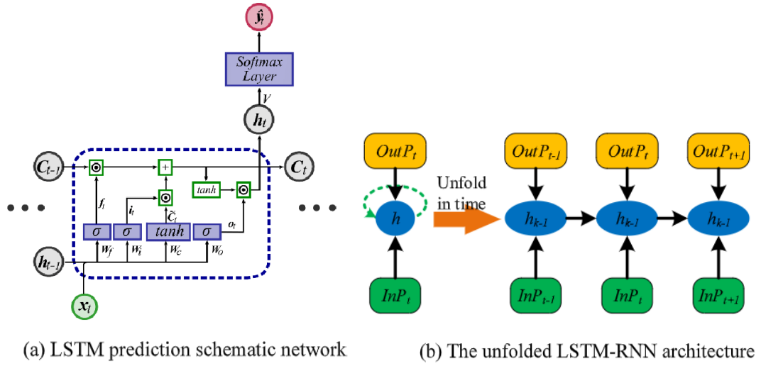
Figure 5 The architectural flow of the LSTM-based prediction network (Bermudez et al., 2017, Wang et al., 2021)
