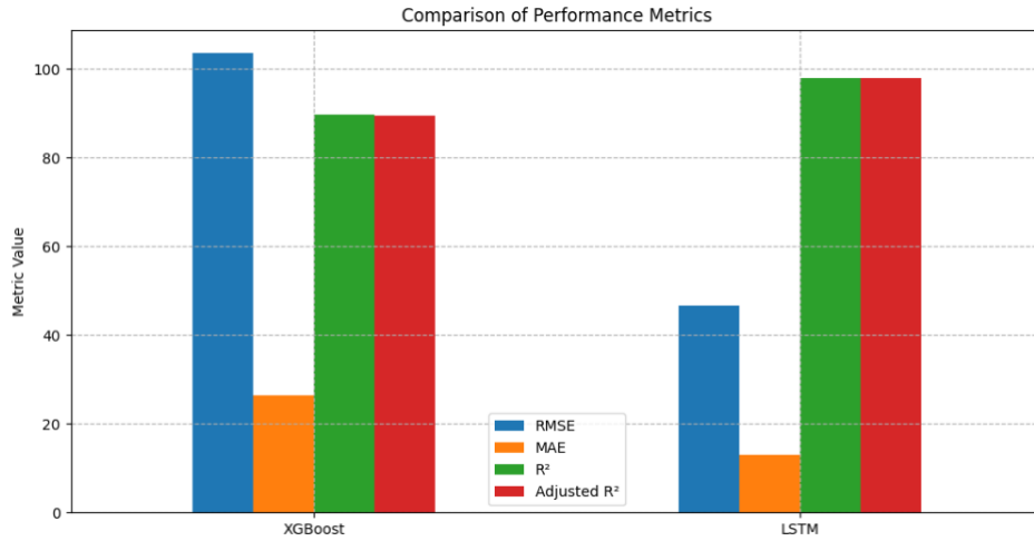
Figure 31 Comparison of Performance Metrics
