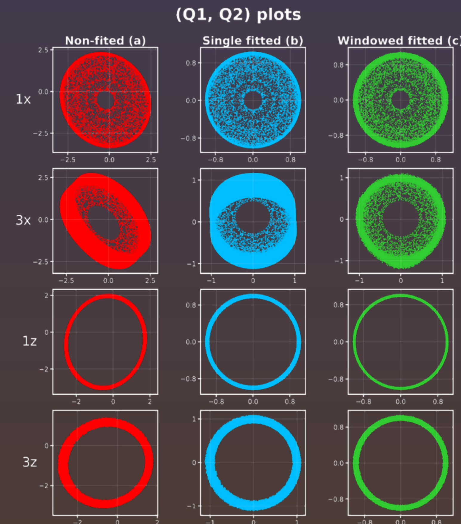
Fig. 4: (Q1, Q2) plots for four HoQIs (1x, 3x, 1z and 3z), comparing (a) the non-fitted, (b) the single ellipse fitted, and (c) the windowed ellipse fitted data.
