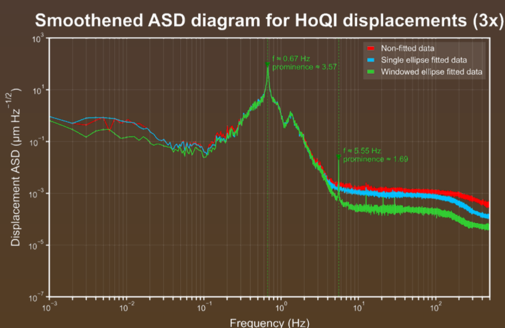
Fig. 6: Smoothed ASD diagram for the displacements of HoQI 3x, comparing the three different data processing approaches.
