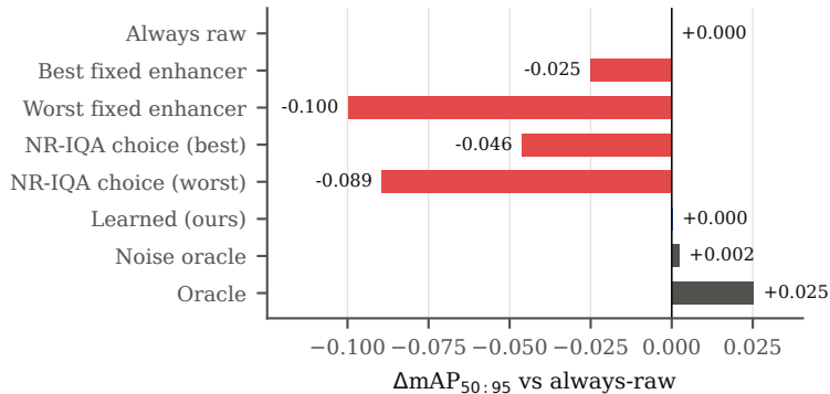
RUOD pred-test (in-domain)
