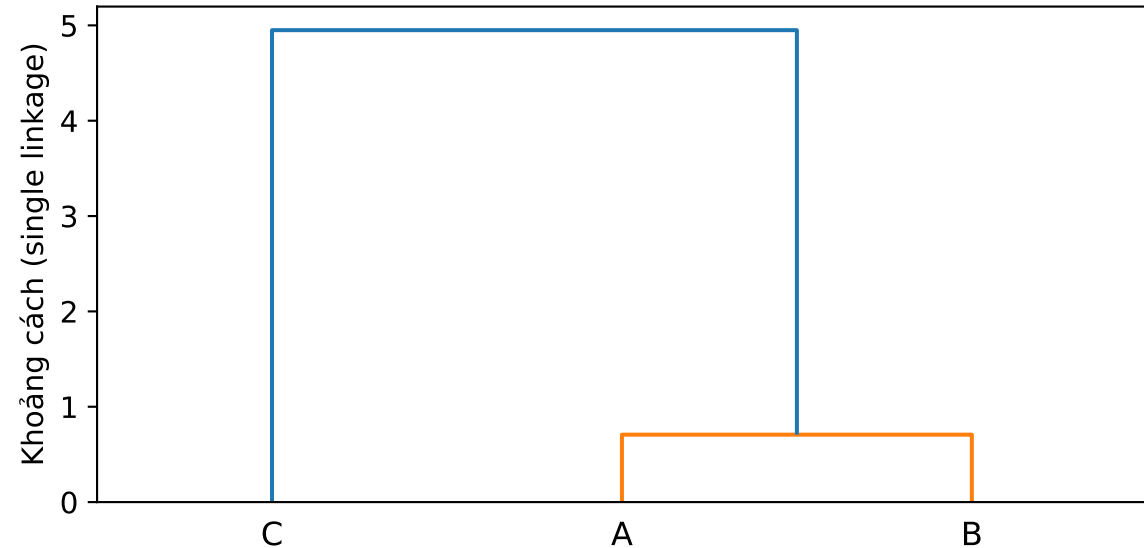
Dendrogram — Euclidean, single linkage (A, B, C)
