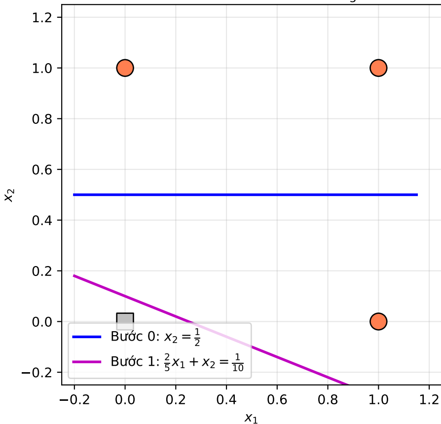
Perceptron GD batch, \rho = \frac{2}{5}
