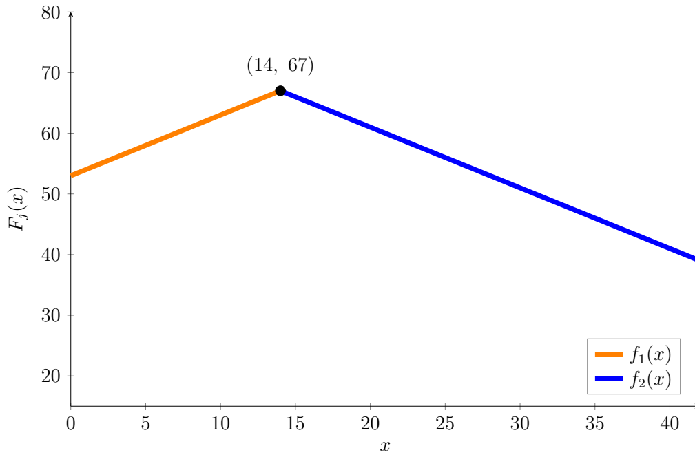
Hình 2.2: Intersection of f_1(x) = x + 53 and f_2(x) = -x + 81
