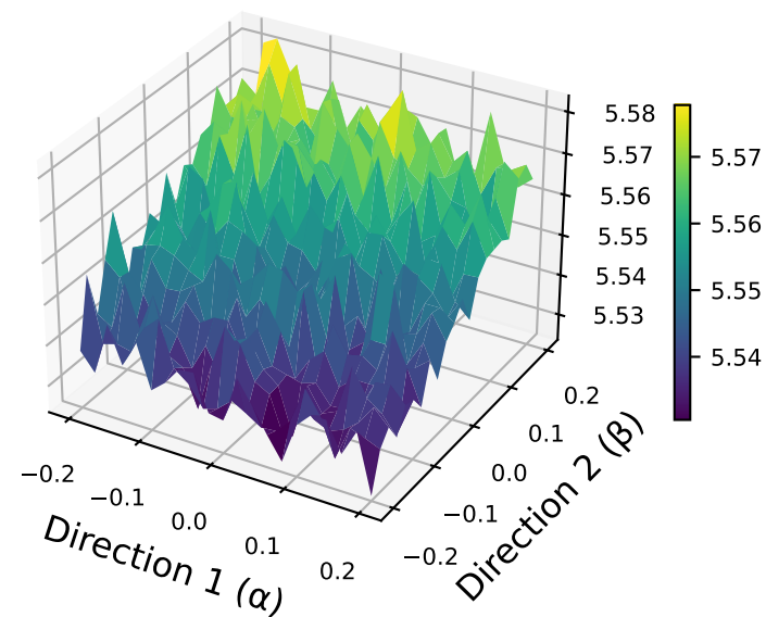
(c) Initial PISSA
