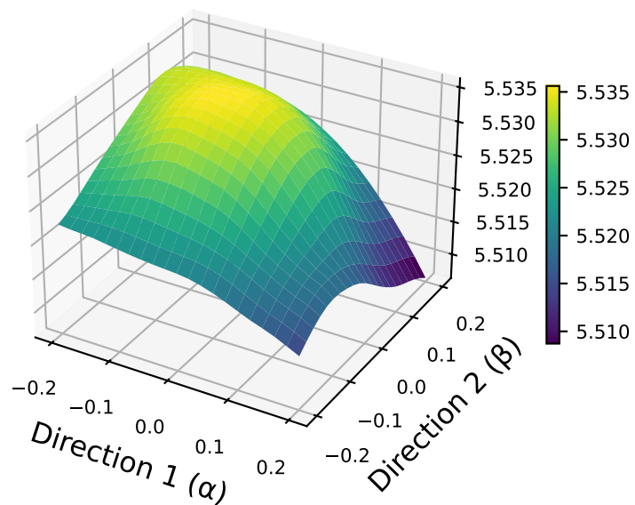
(a) Initial Full Fine-tune
