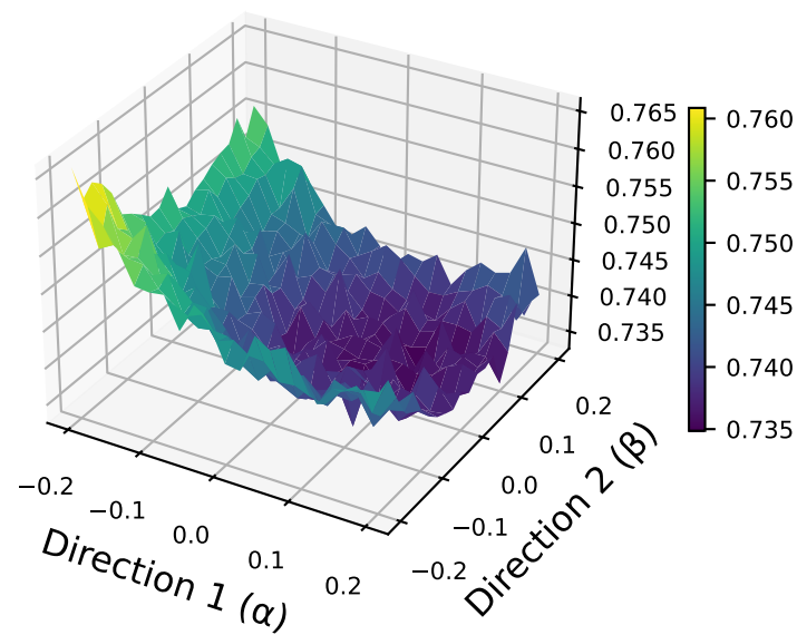
(f) Trained LoRA
