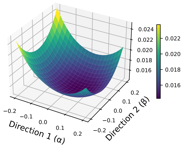
(e) Trained Full Fine-tune
