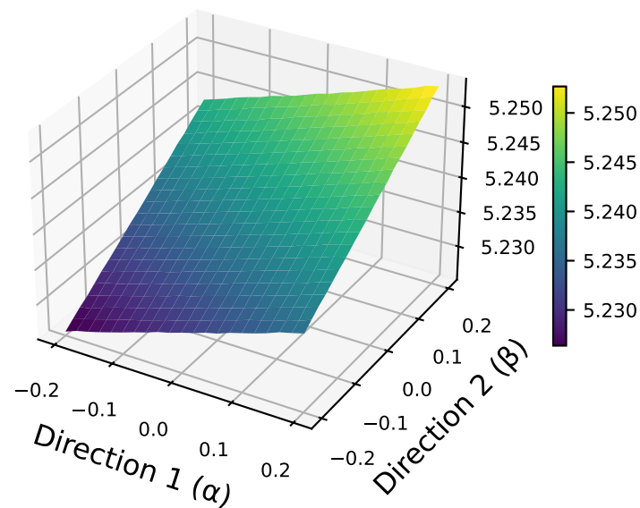
(b) Initial LoRA
