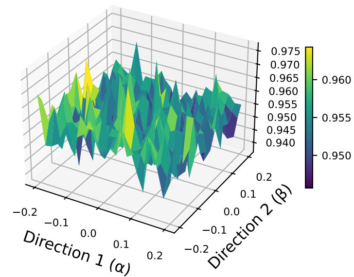
(h) Trained VERA
