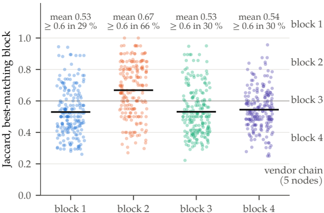
(a) membership stability, 200 weight perturbations
