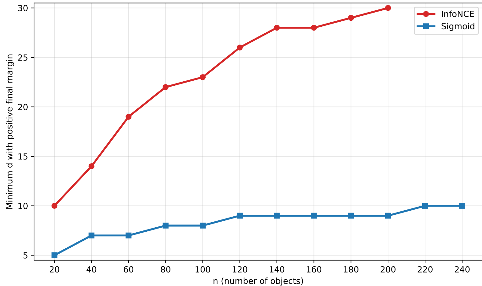
k=2: minimum dimension with positive margin after 100000 steps
