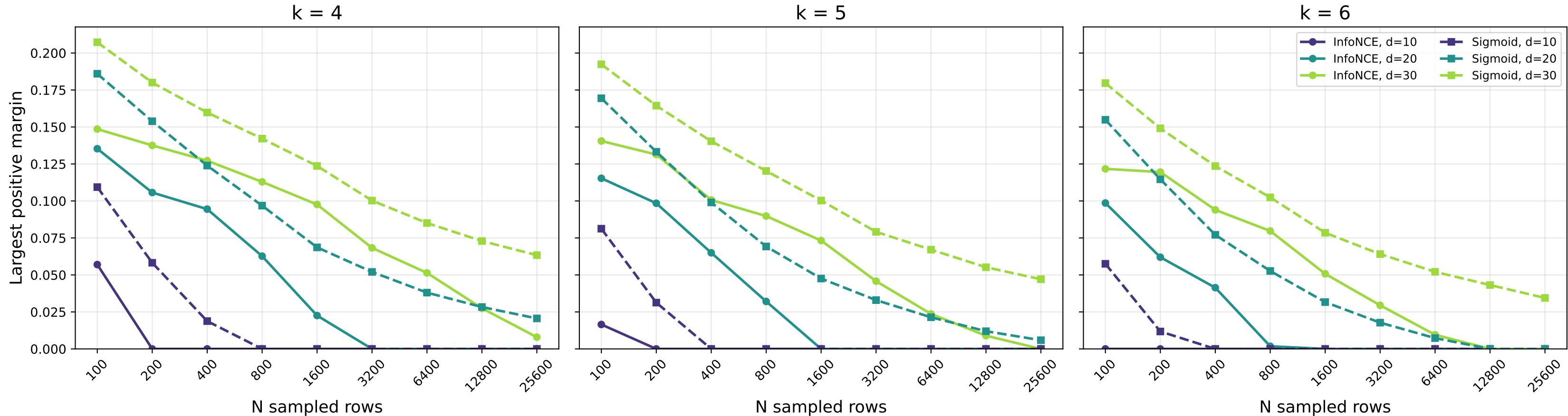
Maximal margin during 100000 steps, fixed iid matrices, n = 100
