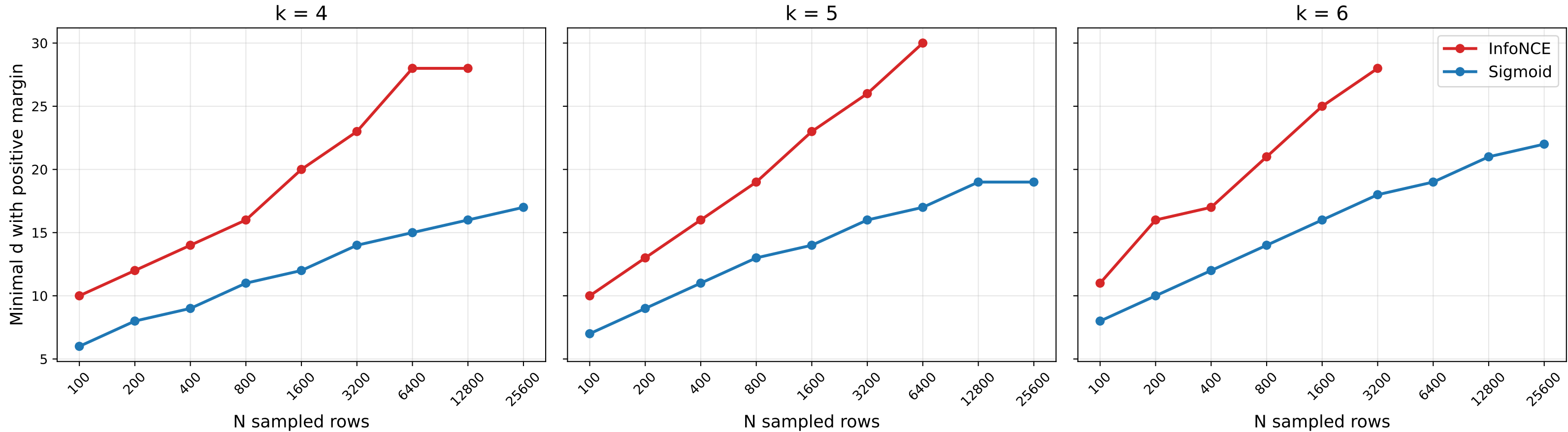
Fixed iid sampled k-sparse matrices, n = 100 (seed 0)
