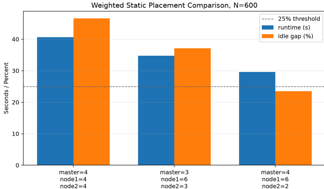
Weighted static placement comparison
