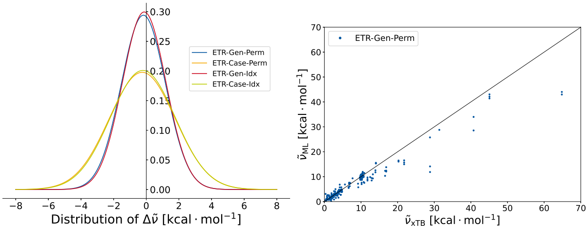
Figure 4.5: On the left is the distribution of \Delta\tilde{\nu} for different models. In every model, the Extra Tree Regression was used. The distribution is assumed to be Gaussian type. For this the median and standard deviation of \Delta\tilde{\nu} are computed. On the right is the \tilde{\nu}_{ML} plotted against \tilde{\nu}_{xTB} . The wave numbers are predicted with the ETR-Gen-Perm model.
