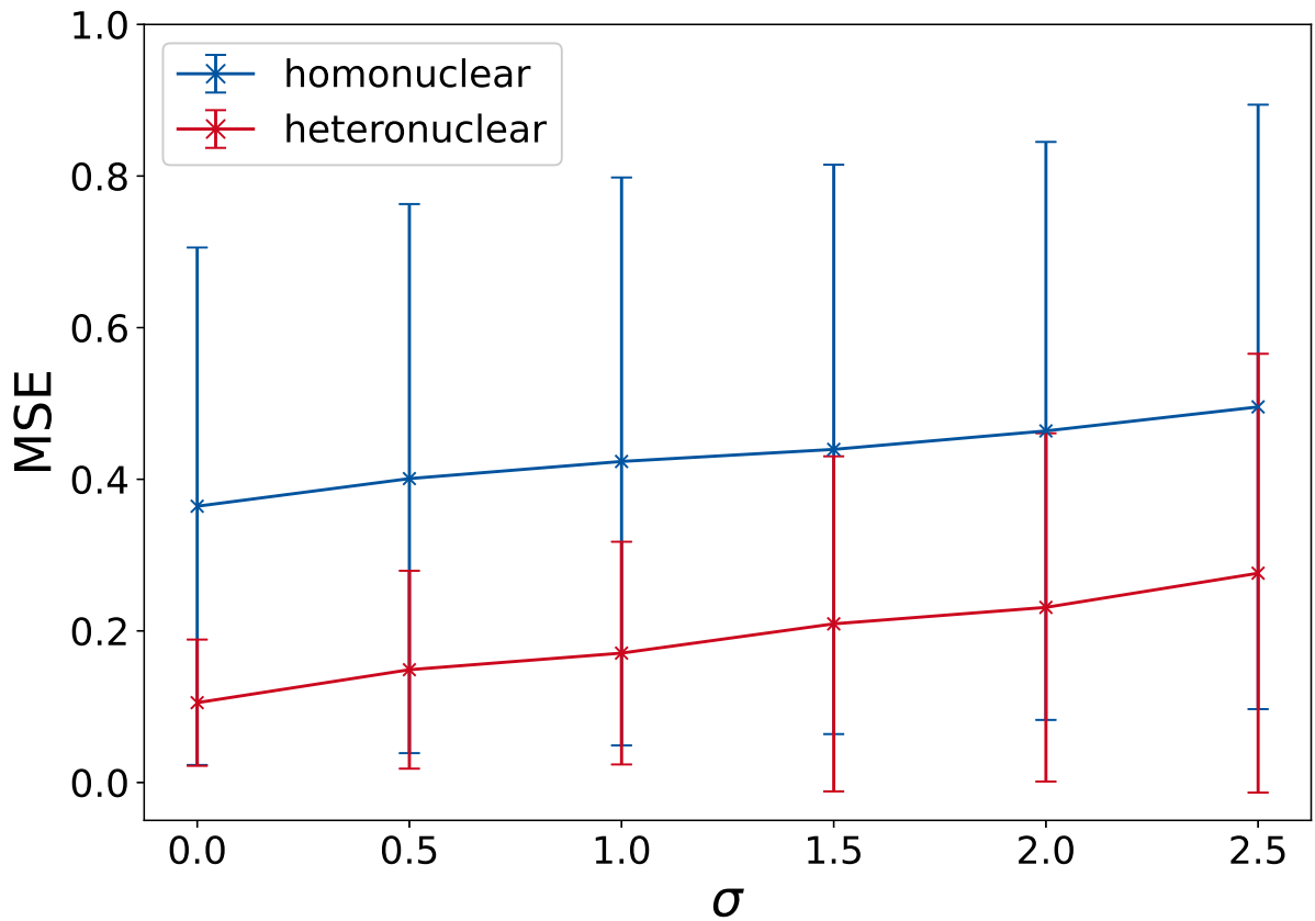
Figure 4.3: Learning plots for predicting hessian elements \frac{\partial^2 E}{\partial a \partial b} for a variation of the factor \sigma . The full sample set, excluding the \text{H}_3 system, is used for the ML models. The mean of ten random states were used for the MSE. The plots are done for the homonuclear model (blue) and heteronuclear model (red).
