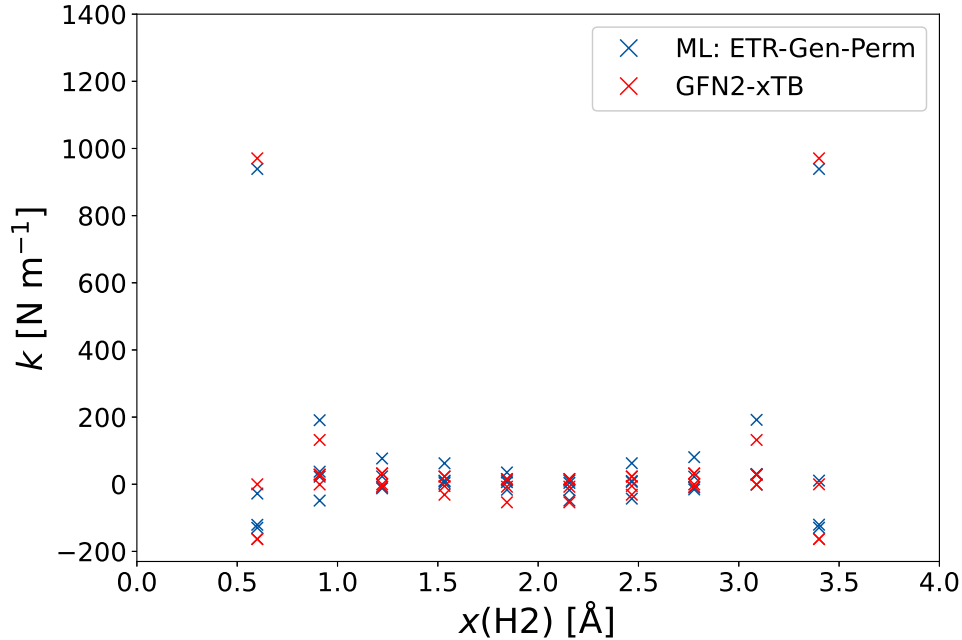
Figure 4.7: Force constants predicted for the \text{H}_3 systems in dependence of the distance between H1 and H2 are shown. The force constants are shown for the GFN2-xTB calculation (red), as also the via the ML model predicted values (blue). The full sample set, excluding the \text{H}_3 system, was used for the ML model. The ML model ETR-Gen-Perm was used for the prediction.
