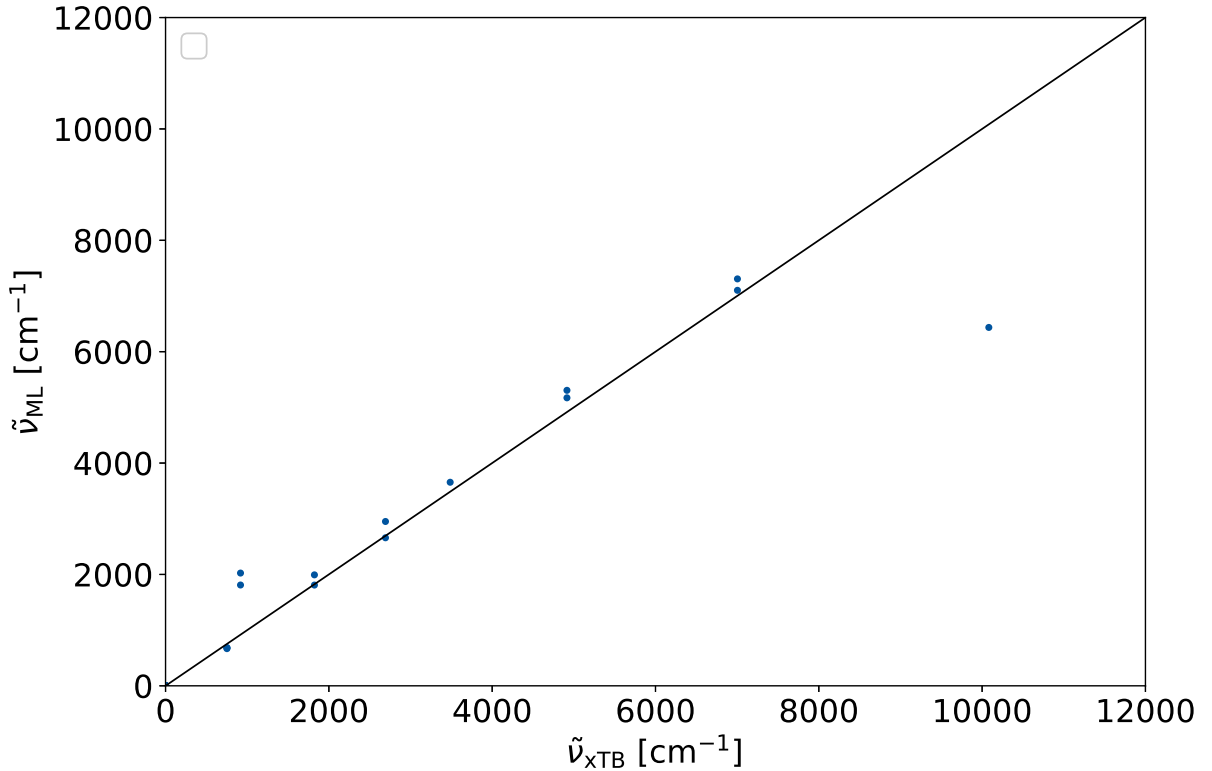
Figure 4.1: The wavenumber, predicted via the ML model \tilde{\nu}_{\text{ML}} is plotted against the wavenumber calculated via GFN2–xTB \tilde{\nu}_{\text{xTB}} . The model uses the Extra Tree Regression. The sample set is H 2 and the training set is 75 % of the whole set. The prediction were done for 5 random states.
