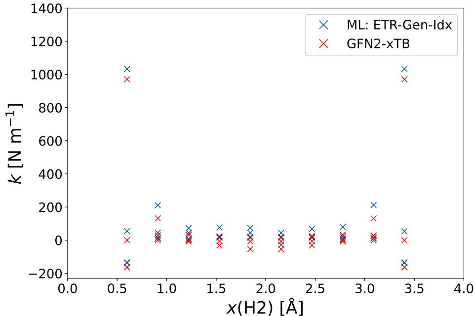
Figure 4.6: Force constants predicted for the H 3 systems in dependence of the distance between H1 and H2 are shown. The force constants are shown for the GFN2-xTB calculation (red), as also the via the ML model predicted values (blue). The full sample set, excluding the H 3 system, was used for the ML model. The ML model ETR-Gen-Idx was used for the prediction.
