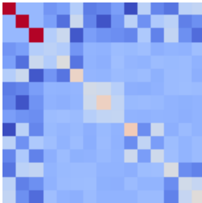
Hessian by GFN2-xTB
