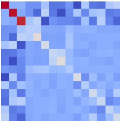
Predicted Hessian
