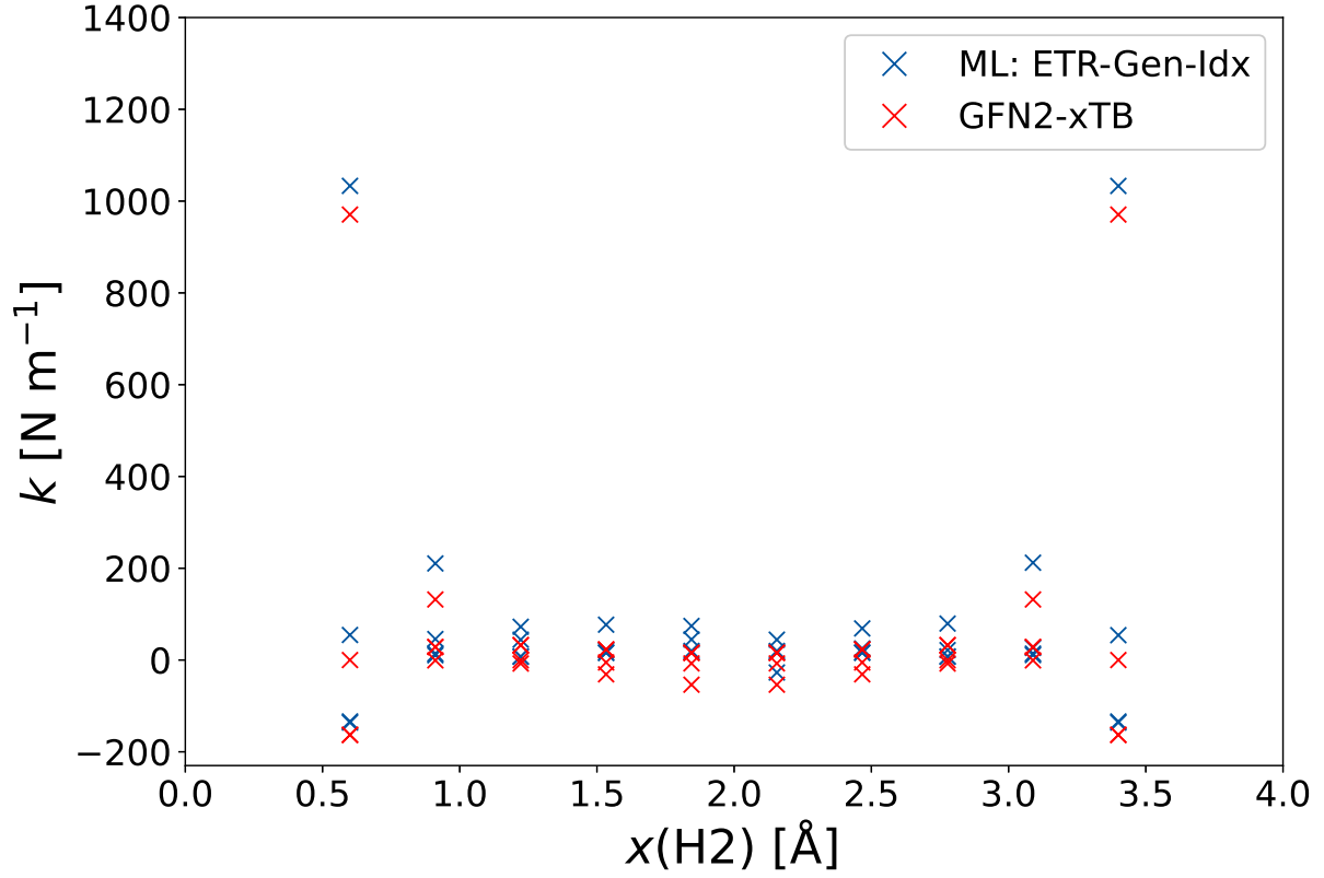
Figure 5.6: Force constants predicted for the \text{H}_3 systems in dependence of the distance between H1 and H2 are shown. The force constants are shown for the GFN2-xTB calculation (red), as also the via the ML model predicted values (blue). The full sample set, excluding the \text{H}_3 system, was used for the ML model. The ML model ETR-Gen-Idx was used for the prediction.
