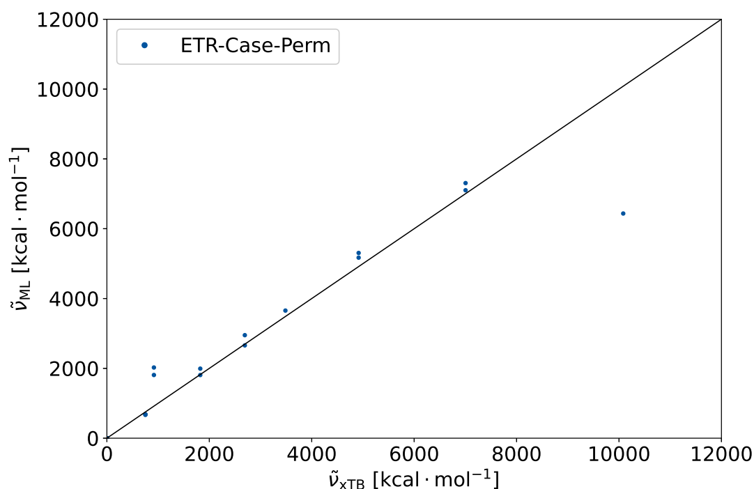
Figure 4.3: The wave number, predicted via the ML model \tilde{\nu}_{\text{ML}} is plotted against the wave number calculated via GFN2–xTB \tilde{\nu}_{\text{xTB}} . The model uses the Extra Tree Regression. The sample set is H 2 and the training set is 75 % of the whole set. The prediction are done for 5 random states.
