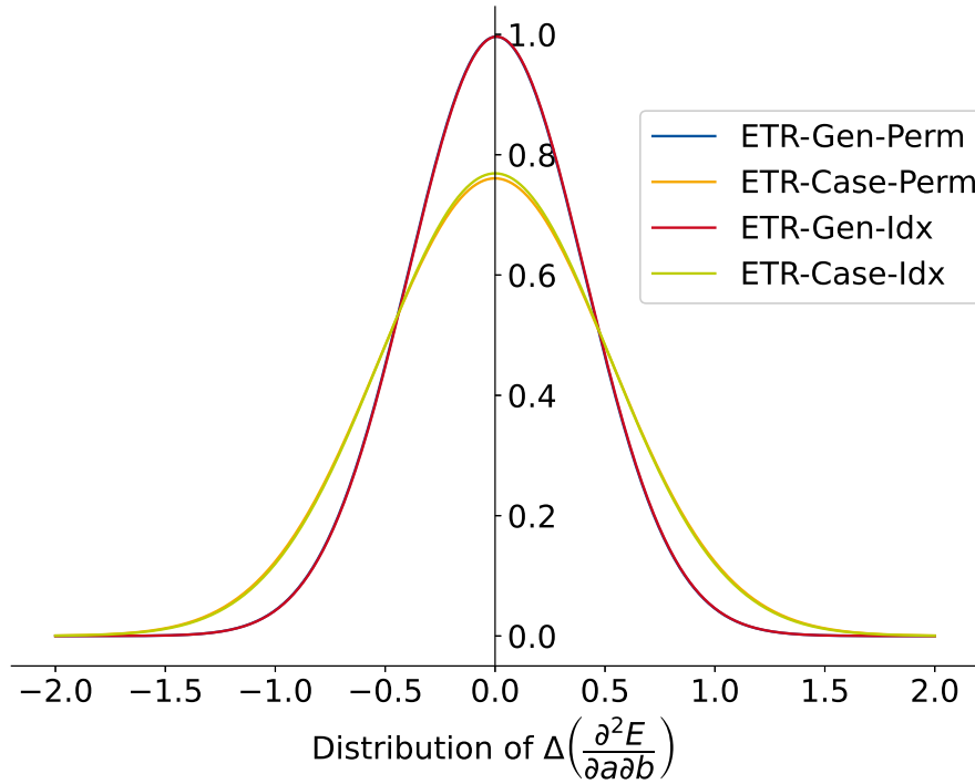
Figure 4.6: Distribution of \Delta\left(\frac{\partial^2 E}{\partial a \partial b}\right) for different models. In every model, the ETR is used. The distribution is assumed to be Gaussian. For this the median and standard deviation of \Delta\left(\frac{\partial^2 E}{\partial a \partial b}\right) are computed.
