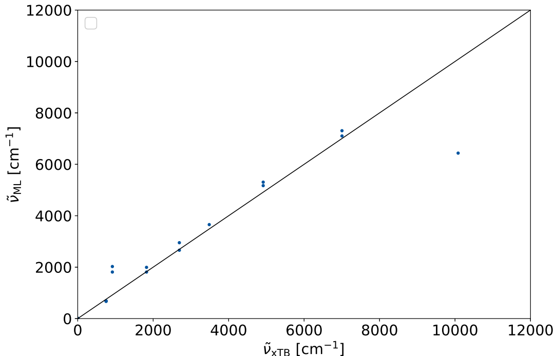
Figure 4.2: The wavenumber, predicted via the ML model \tilde{\nu}_{\text{ML}} is plotted against the wave number calculated via GFN2–xTB \tilde{\nu}_{\text{xTB}} . The model uses the Extra Tree Regression. The sample set is \text{H}_2 and the training set is 75 % of the whole set. The prediction were done for 5 random states.
