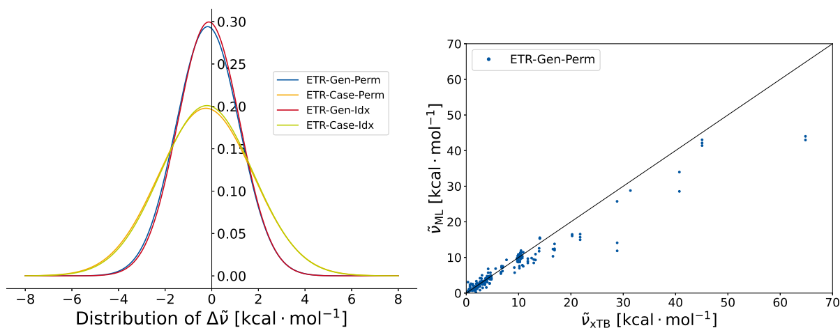
Figure 4.6: On the left is the distribution of \Delta\tilde{\nu} for different models. In every model, the Extra Tree Regression was used. The distribution is assumed to be Gaussian type. For this the median and standard deviation of \Delta\tilde{\nu} are computed. On the right is the \tilde{\nu}_{ML} plotted against \tilde{\nu}_{xTB} . The wave numbers are predicted with the ETR-Gen-Perm model.
