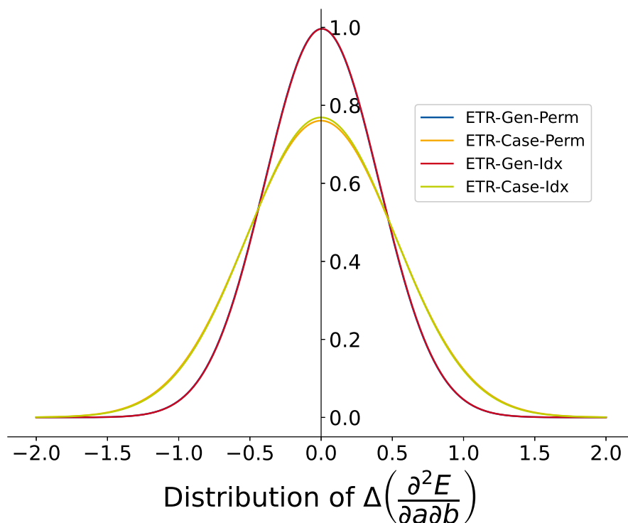
Figure 4.5: Distribution of \Delta\left(\frac{\partial^2 E}{\partial a \partial b}\right) for different models. In every model, the Extra Tree Regression was used. The distribution is assumed to be Gaussian type. For this the median and standard deviation of \Delta\left(\frac{\partial^2 E}{\partial a \partial b}\right) are computed.
