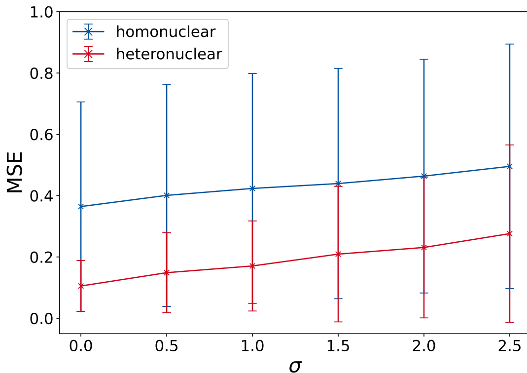
Figure 4.4: Learning plots for predicting hessian elements \frac{\partial^2 E}{\partial a \partial b} for a variation of the factor \sigma . The full sample set, excluding the H_3 system, is used for the ML models. The mean of ten random states were used for the MSE. The plots are done for the homonuclear model (blue) and heteronuclear model (red).
