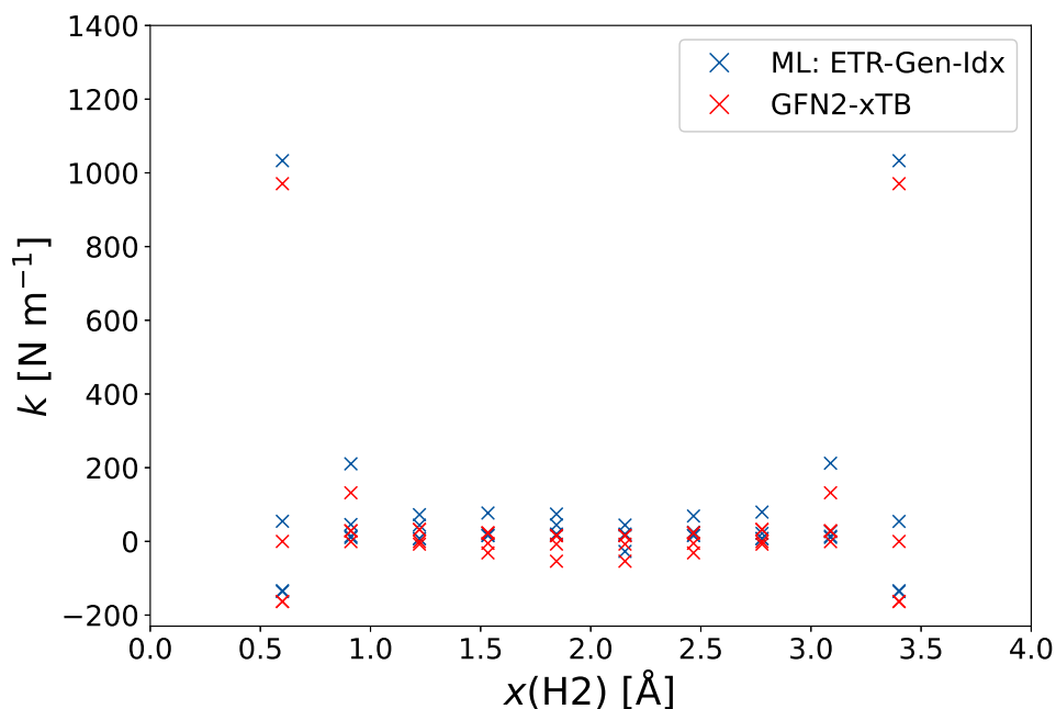
Figure 4.7: Force constants predicted for the H 3 systems in dependence of the distance between H1 and H2 are shown. The force constants are shown for the GFN2-xTB calculation (red), as also the via the ML model predicted values (blue). The full sample set, excluding the H 3 system, was used for the ML model. The ML model ETR-Gen-Idx was used for the prediction.
