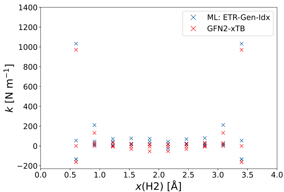
Figure 4.8: Force constants of the \text{H}_3 system as a function of the distance between H1 and H2. H1 is located at x(\text{H1}) = 0.0 \text{ \AA} and H3 at x(\text{H3}) = 4.0 \text{ \AA} . The force constants are shown for the GFN2-xTB calculation (red), and the predicted values (blue). The full sample set, excluding the \text{H}_3 system, is used for the ML model. The ML model ETR-Gen-Idx is used for the prediction.
