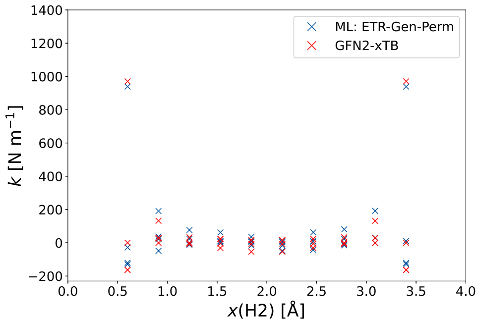
Figure 4.9: Force constants of the \text{H}_3 system as a function of the distance between H1 and H2. H1 is located at x(\text{H1}) = 0.0 \text{ \AA} and H3 at x(\text{H3}) = 4.0 \text{ \AA} . The force constants are shown for the GFN2-xTB calculation (red), and the predicted values (blue). The full sample set, excluding the \text{H}_3 system, is used for the ML model. The ML model ETR-Gen-Perm is used for the prediction.
