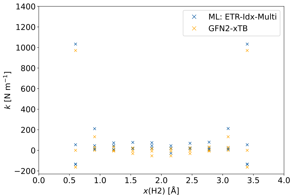
Figure 5.9: Force constants predicted for the \text{H}_3 systems in dependence of the distance between H1 and H2 are shown. The force constants are shown for the GFN2-xTB calculation (yellow), as also the via the ML model predicted values (blue). The full sample set, excluding the \text{H}_3 system, was used for the ML model. The ML model indexed; multi was used for the prediction.
