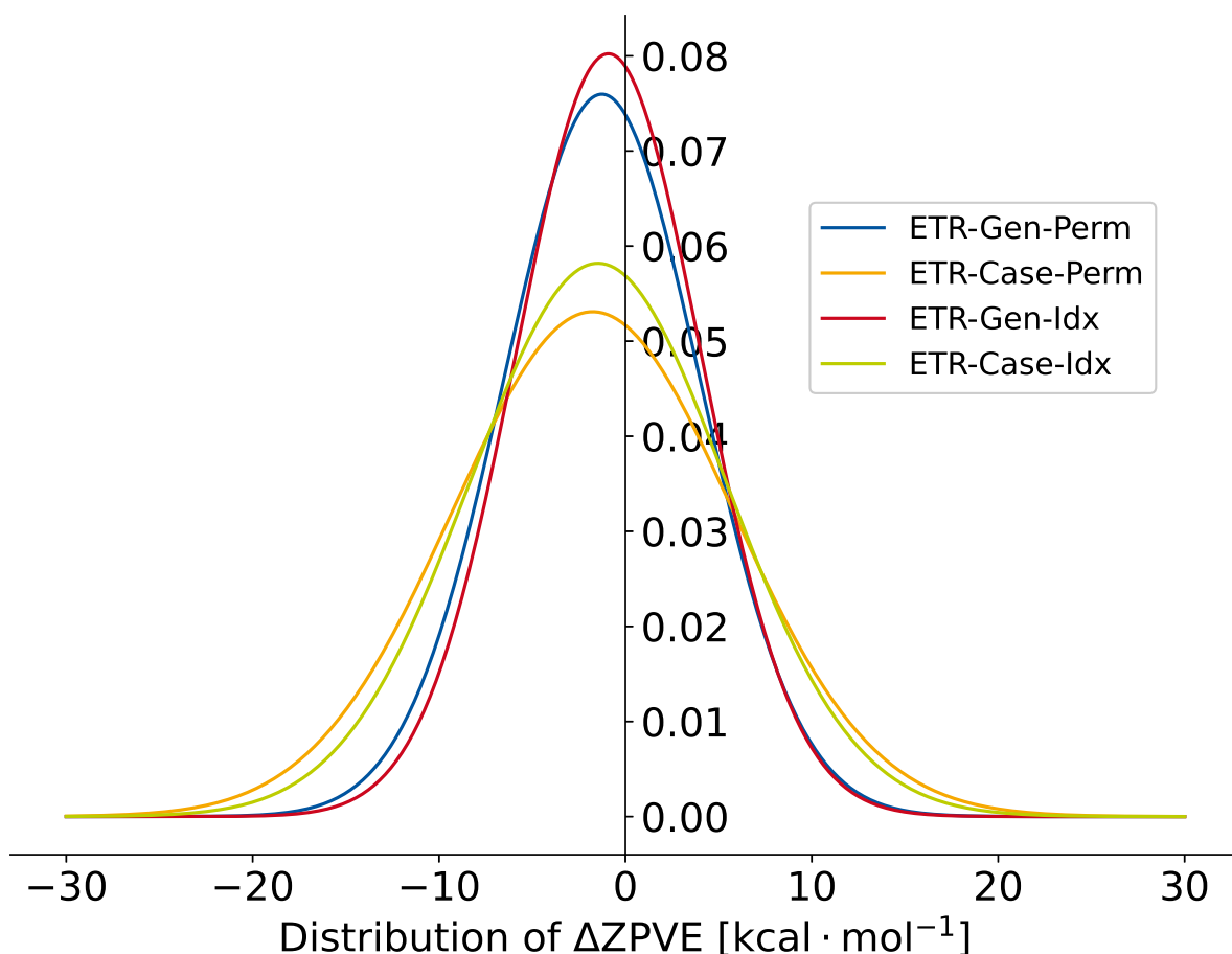
Figure 5.8: Distribution of \Delta ZPE for different models. In every model, the Extra Tree Regression was used. The distribution is assumed to be Gaussian type. For this the median and standard deviation of \Delta ZPE are computed.
