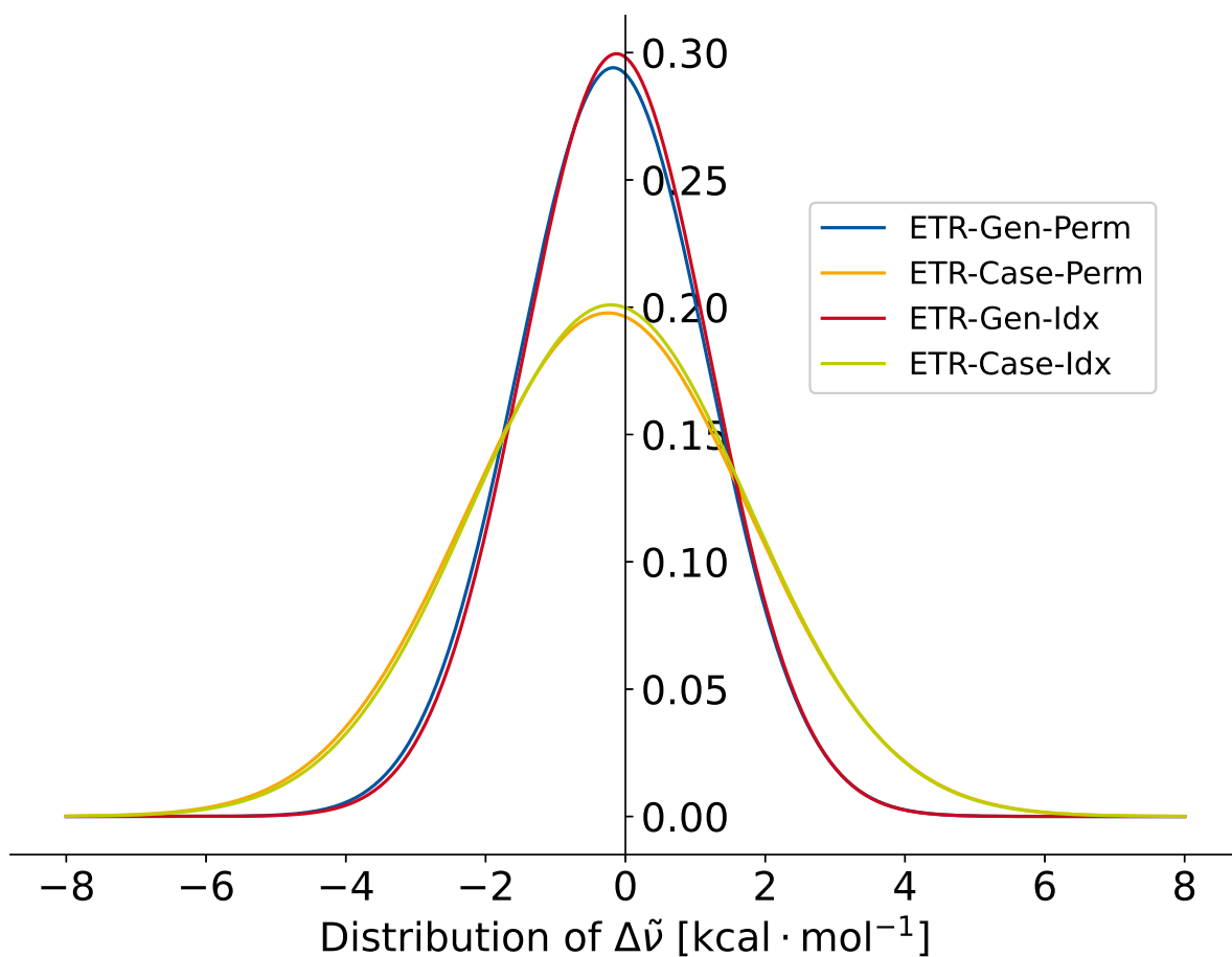
Figure 5.7: Distribution of \Delta\tilde{\nu} for different models. In every model, the Extra Tree Regression was used. The distribution is assumed to be Gaussian type. For this the median and standard deviation of \Delta\tilde{\nu} are computed.
