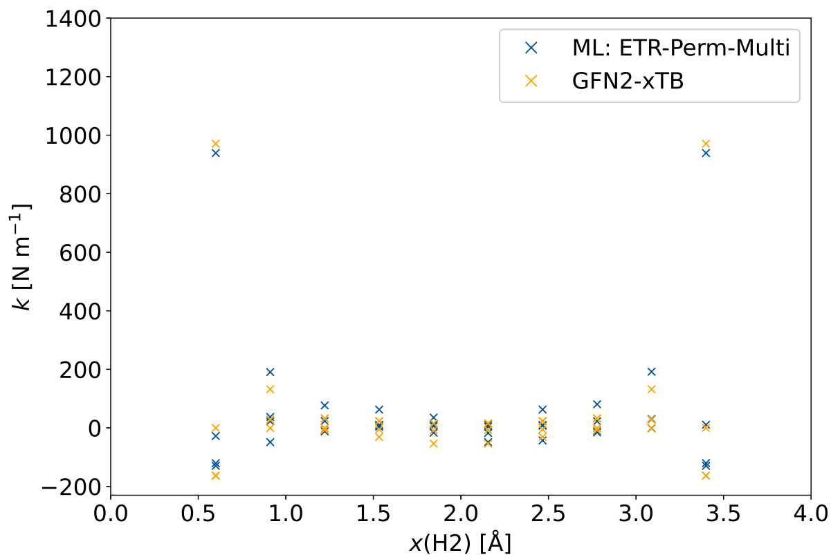
Figure 5.10: Force constants predicted for the \text{H}_3 systems in dependence of the distance between H1 and H2 are shown. The force constants are shown for the GFN2-xTB calculation (yellow), as also the via the ML model predicted values (blue). The full sample set, excluding the \text{H}_3 system, was used for the ML model. The ML model perm; multi was used for the prediction.
