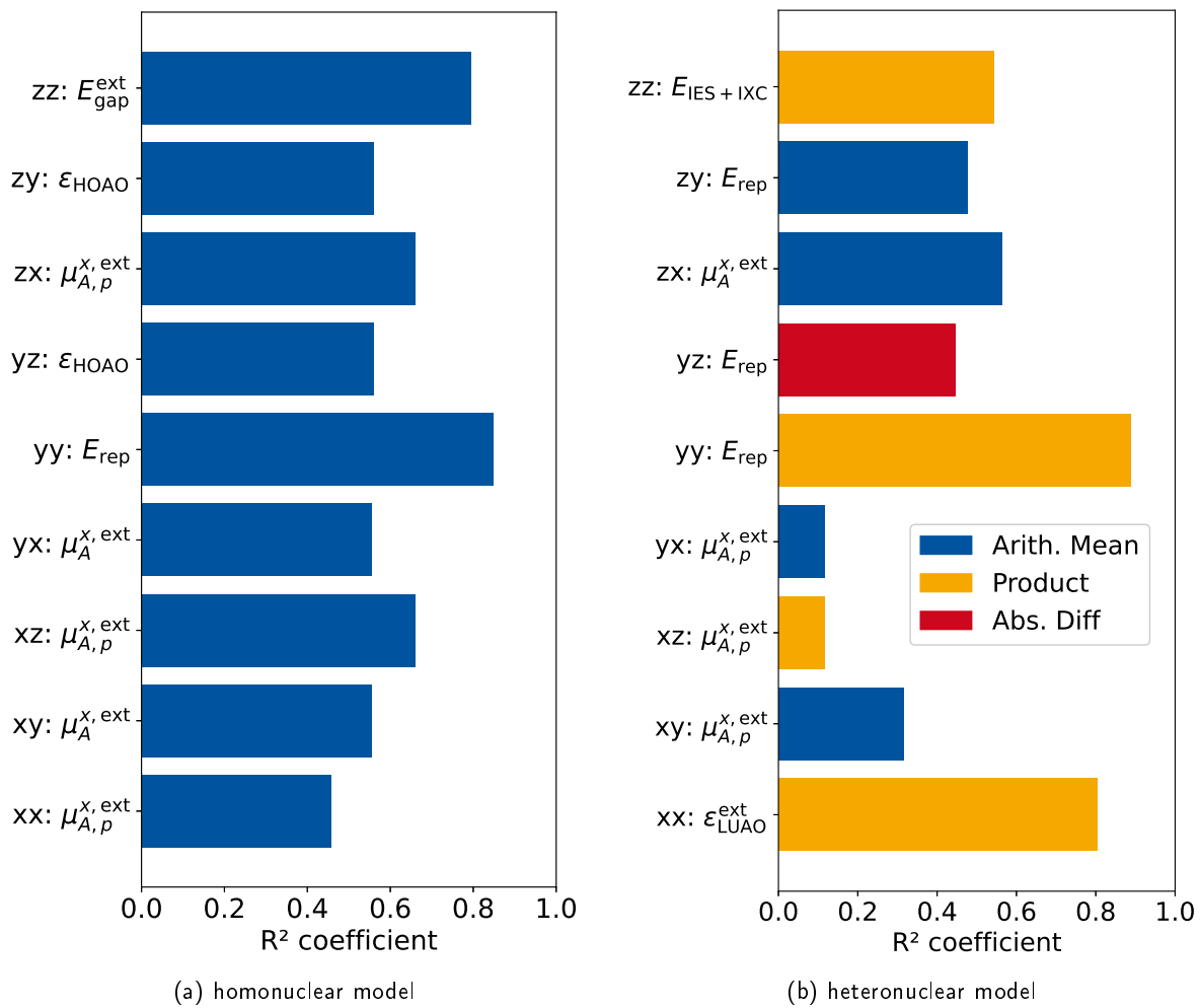
Figure 4.2: Highest Pearson Correlation Coefficient specifically computed for each Hessian element for the homo- and heteronuclear model. The abbreviation ab corresponds to the elements \frac{\partial^2 E}{\partial a_A \partial b_B} .
