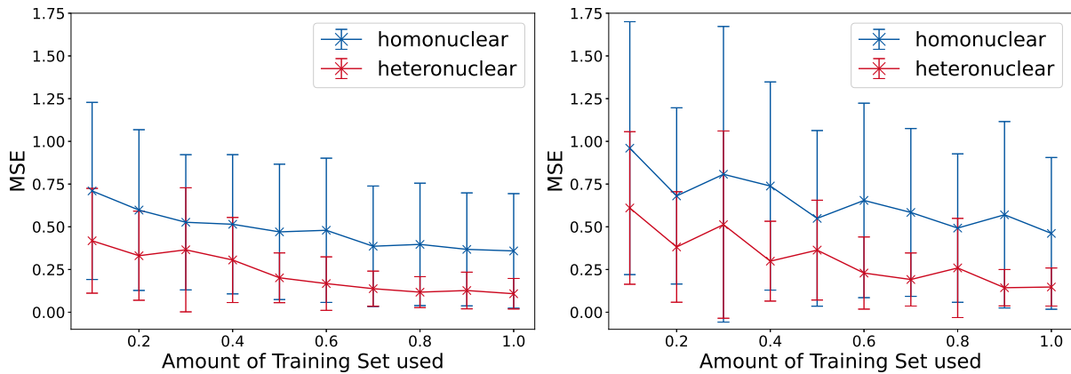
Figure 4.4: Learning plots for the predicting Hessian elements \frac{\partial^2 E}{\partial a \partial b} for an increase of the amount of training set used. On the left is the learning plot of the Extra Tree Regression and on the right the plot of the Random Forest Regression shown. The full training set is 75 % of the sample set. The full sample set, excluding the H_3 system, is used. The mean of ten random states were used for the MSE. The plots are done for the homonuclear model (blue) and heteronuclear model (red).
