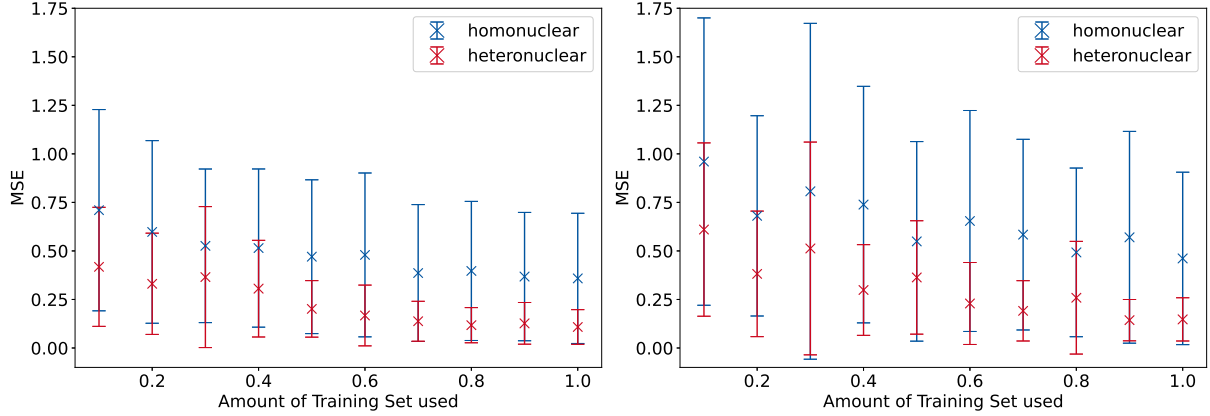
Figure 5.2: Learning plots for the predicting hessian elements \frac{\partial^2 H}{\partial a \partial b} for an increase of the amount of training set used. On the left is the learning plot of the Extra Tree Regression and on the right the plot of the Random Forest Regression shown. The full training set is 75 % of the sample set. The full sample set, excluding the H_3 system, is used. The mean of ten random states were used for the MSE. The plots are done for the homonuclear model (blue) and heteronuclear model (red).
