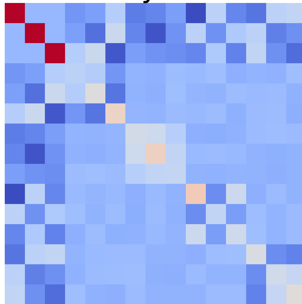
Hessian by GFN2-xTB
