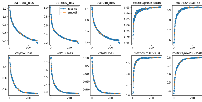
Fig. 3. Training behaviour of the final configuration. Box, classification and distribution-focal losses converge without divergence on either split, and both mAP measures rise monotonically before flattening.
