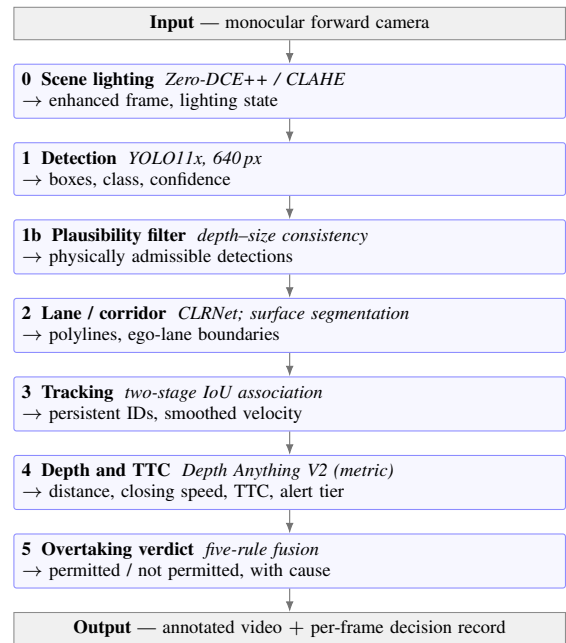
Fig. 1. The six-stage pipeline. Each stage consumes the outputs above it and substitutes a weaker method rather than aborting when its model is unavailable.
