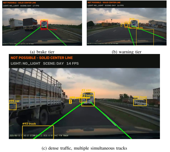
Fig. 4. Pipeline output. (a) and (b) show the two collision alert tiers with distance and time-to-collision; (c) shows simultaneous tracking under dense traffic.
