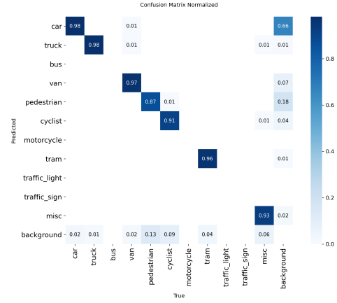
Fig. 2. Normalised confusion matrix on the validation split. Diagonal entries are correct classifications; off-diagonal entries show the categories most often interchanged.
