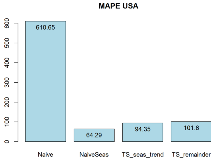
MAPE values for different forecasting models on validation set
