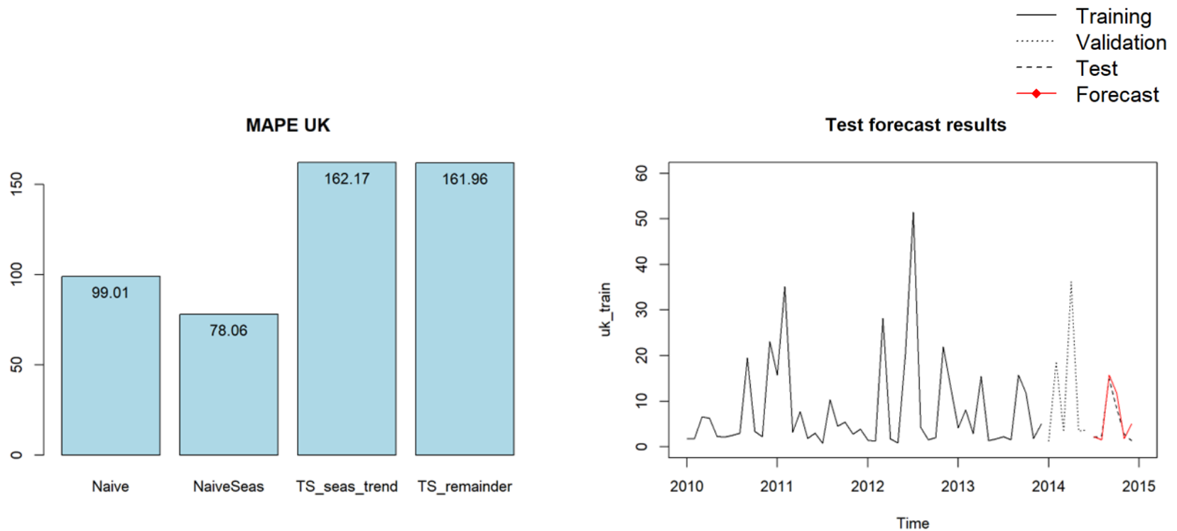
MAPE values for different forecasting models on validation set
