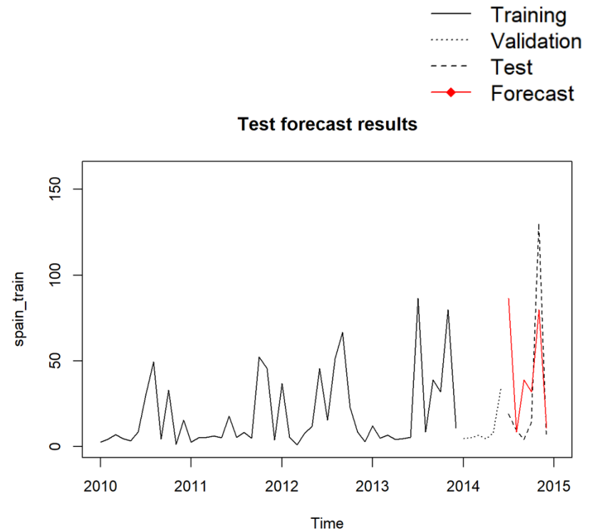
Forecast for test set using Naive Seasonality model
