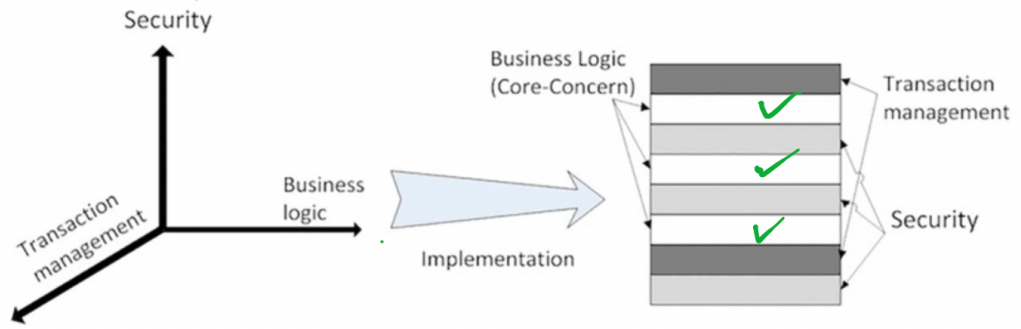
(a) Code tangling
