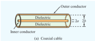
(a) Coaxial cable
