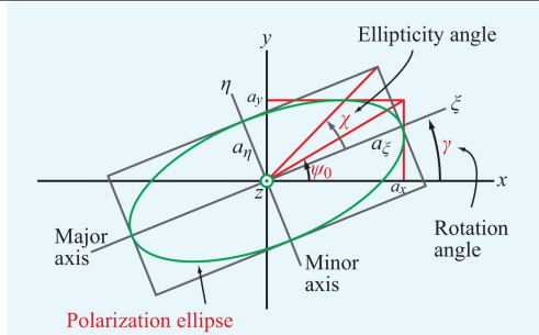
Figure 7-11 Polarization ellipse in the x - y plane with the wave traveling in the z direction (out of the page).
