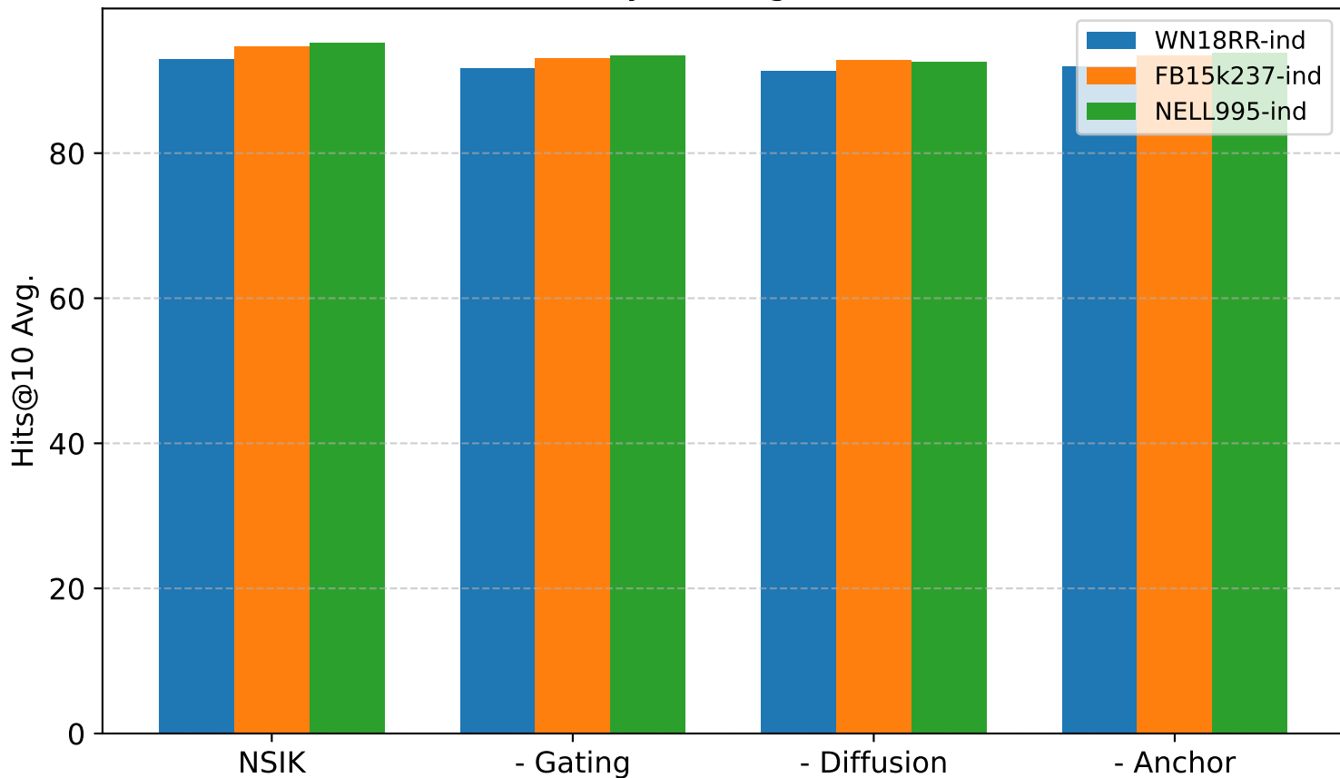
Ablation Study (Average Performance)
