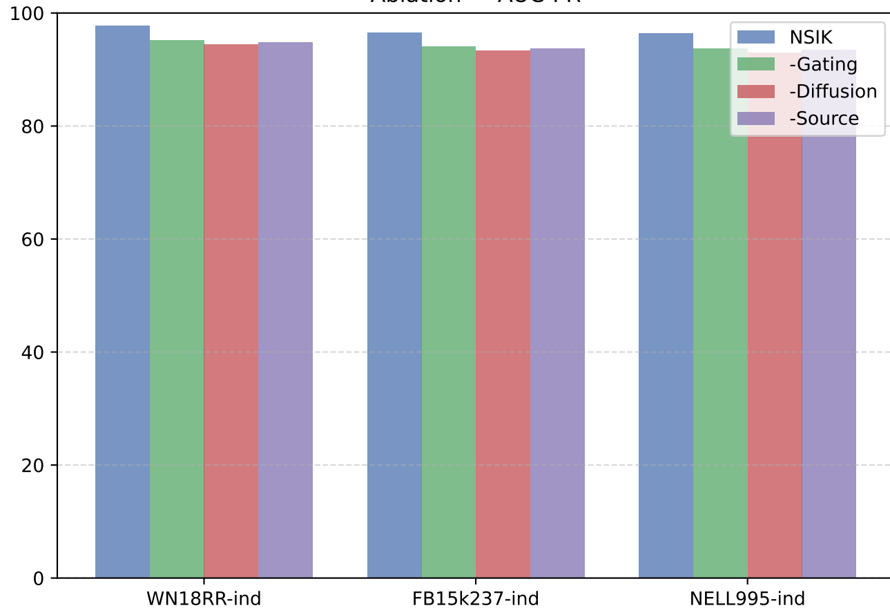
Ablation — AUC-PR
