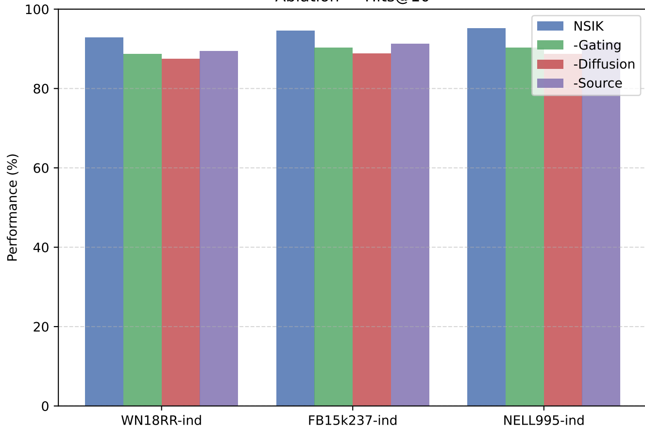
Ablation — Hits@10
