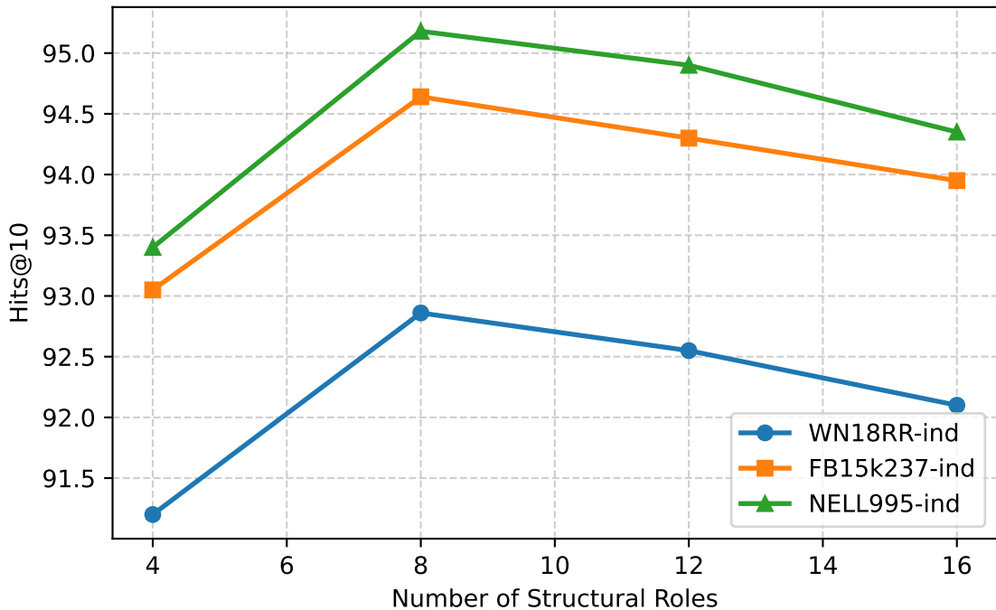
Role Sensitivity Analysis
