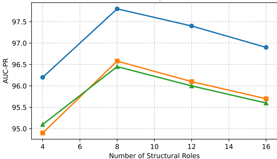
Role Sensitivity — AUC-PR
