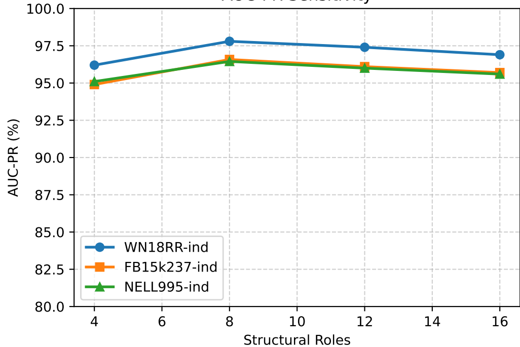
AUC-PR Sensitivity
