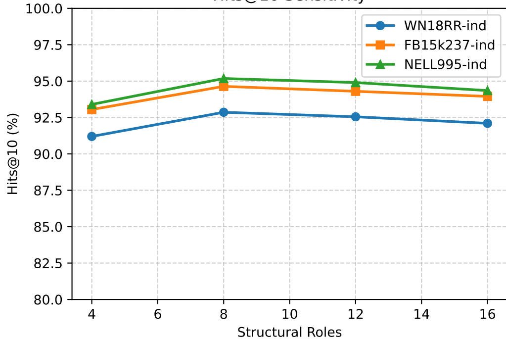
Hits@10 Sensitivity
